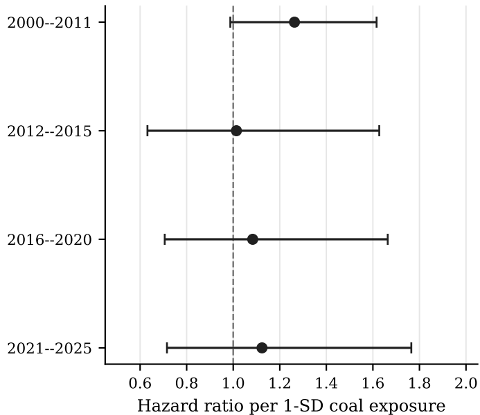
(b) Period-specific Cox estimates
