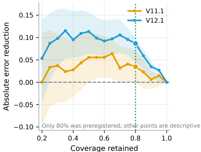
b Routing benefit with 95% CI
