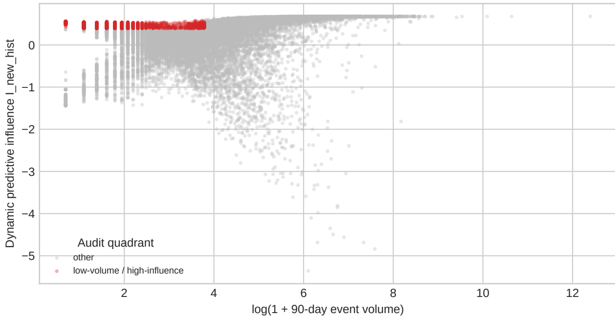
Dynamic predictive influence is not synonymous with volume
