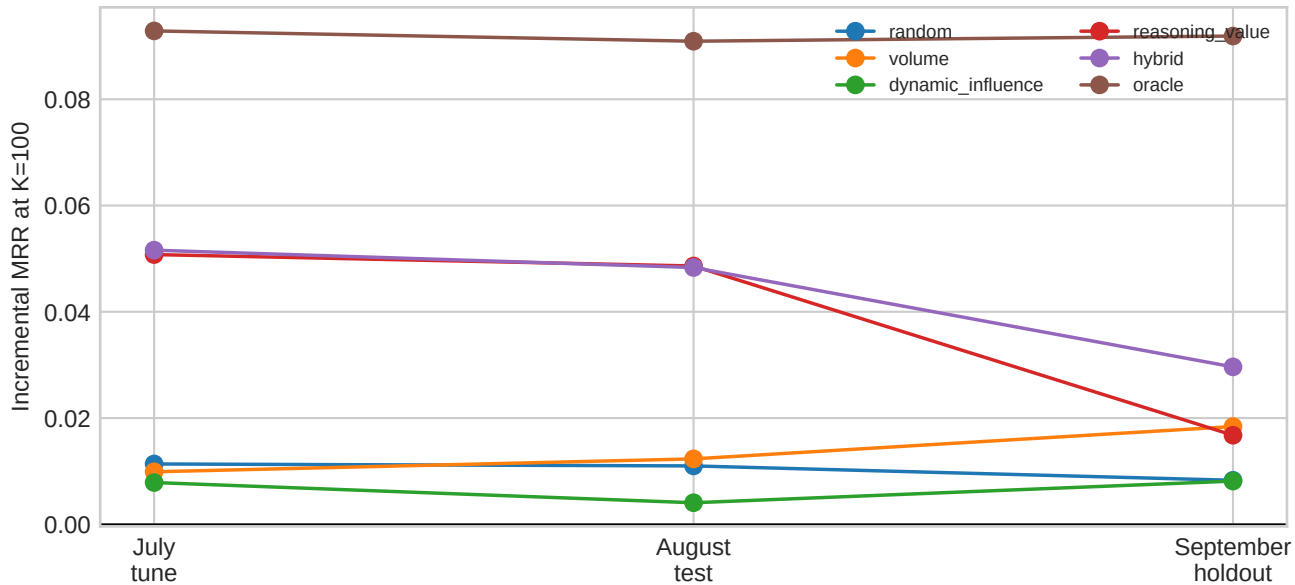
Temporal generalization at the preregistered K=100 budget
