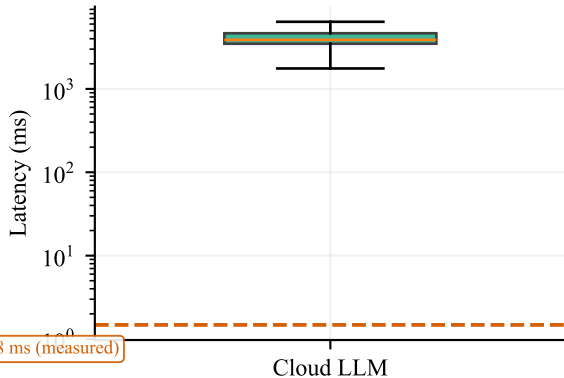
(a) Cloud round-trip latency (real traces)
