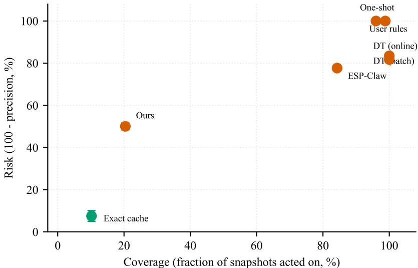
Risk-coverage operating points, pooled UCI replay (1,440 snapshots)
