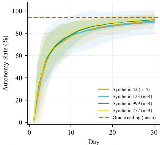
(a) Synthetic 4x repeats
