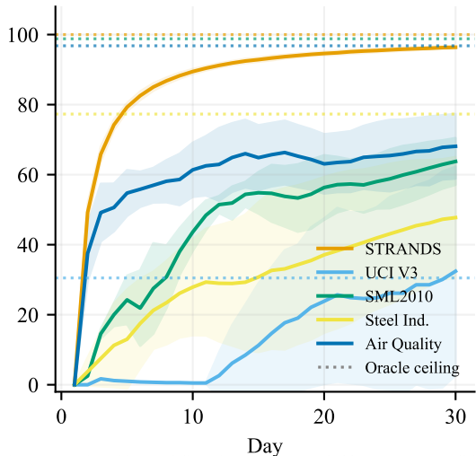
(b) Real datasets (30-day full horizon)
