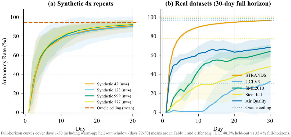
Figure 3: Daily autonomy learning curves over 30 days, per-dataset means across the four seeded runs (36 held-out blocks in total; full-horizon curves include the warm-up, so endpoints differ from the held-out means in Table 1).
