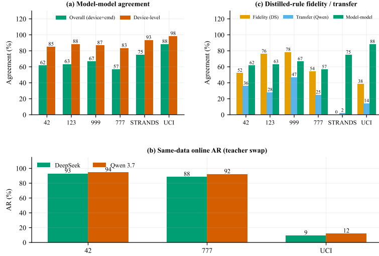
(a) same-prompt DeepSeek-majority vs Qwen on 60 snapshots/dataset; (b) online runs on identical sensor sequences (v10.6 generator fix); (c) same teacher-replay snapshots, original run prompt, engine resolution (device+cmd; device-level in rule_transfer.json).
