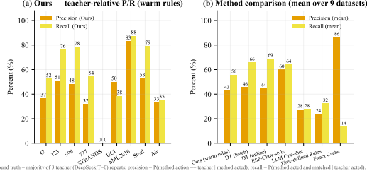
Figure 5: Precision–recall on the 60-snapshot teacher replay: (a) per dataset with the warm-up rule set, (b) method means over nine datasets.
