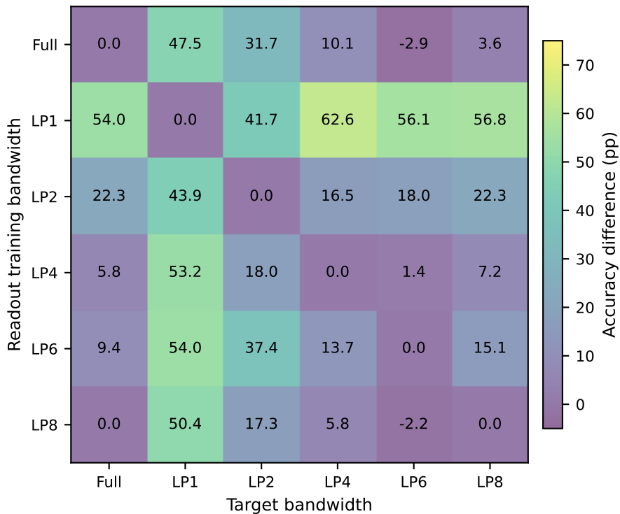
Dogs: target-referenced transfer deficit
