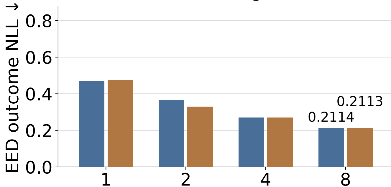
(a) RunBugRun
