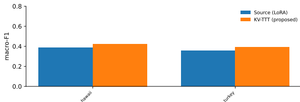
Fig. 1. Macro-F1 of the frozen source vs. KV-TTT per leave-one-event-out fold (bars for completed folds; pending folds omitted).
