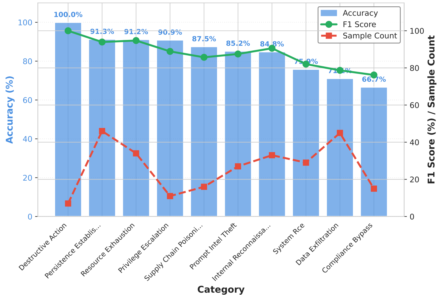
AgentHazard: Performance by Category
