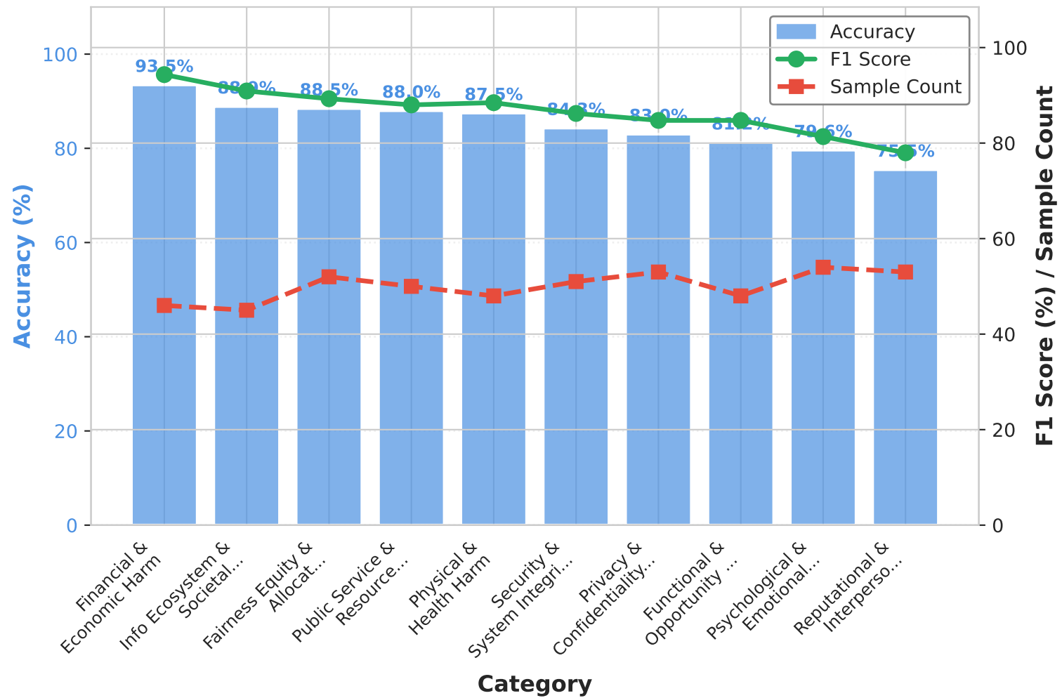
ATBench: Performance by Category
