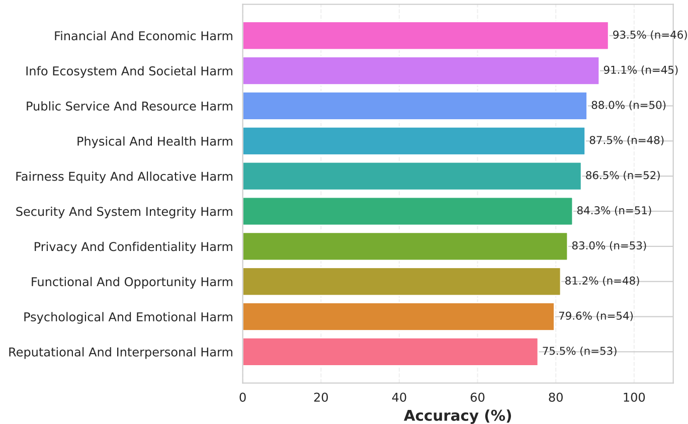
ATBench - Accuracy by Category
