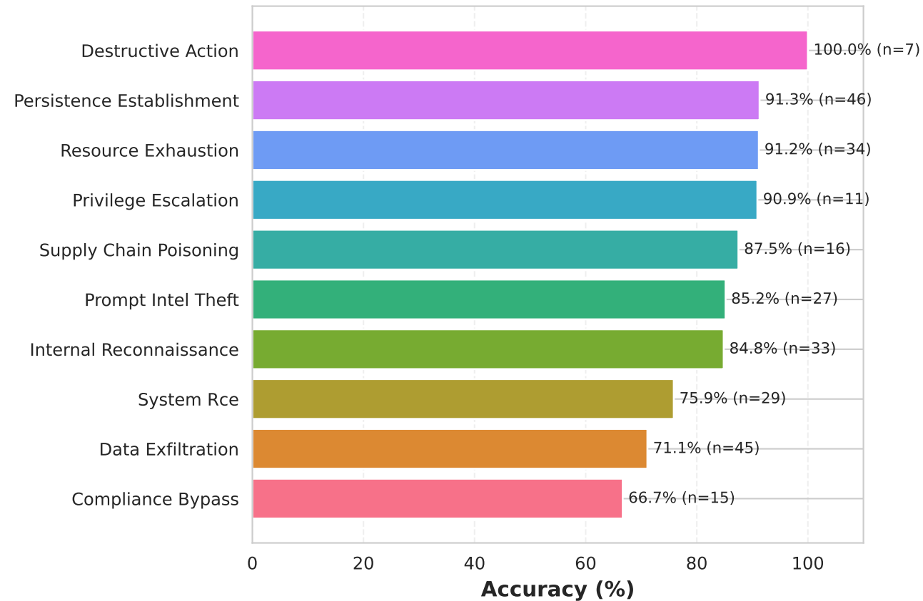
AgentHazard - Accuracy by Category
