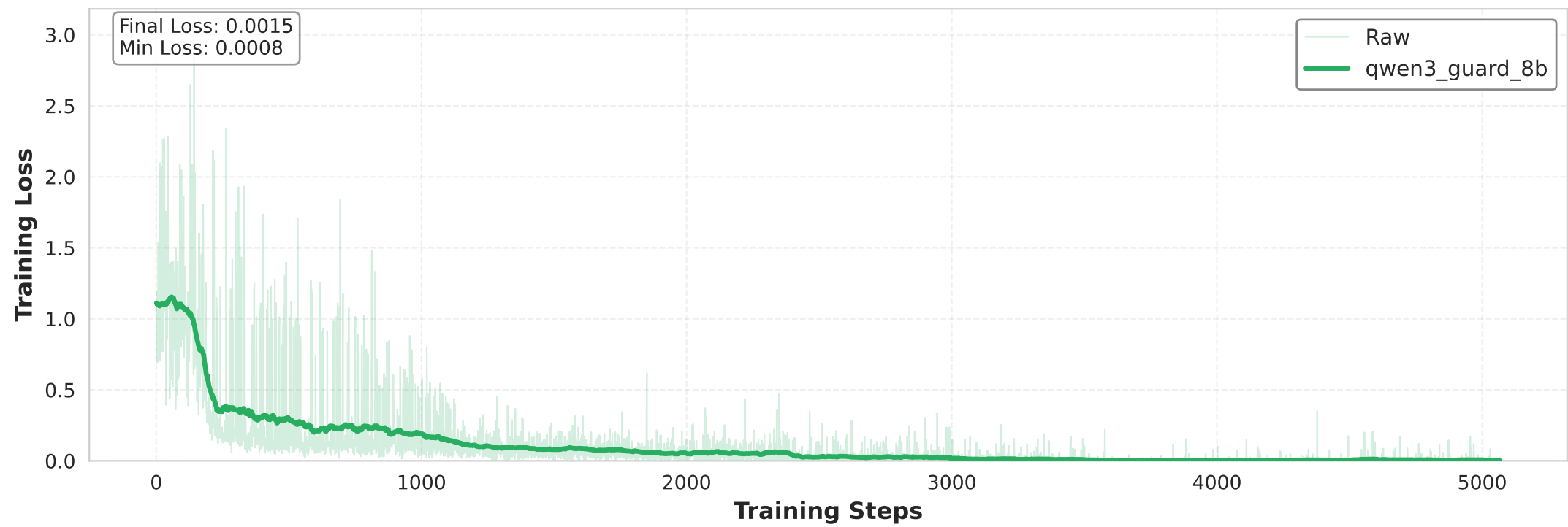
qwen3_guard_8b - Training Loss Curve
