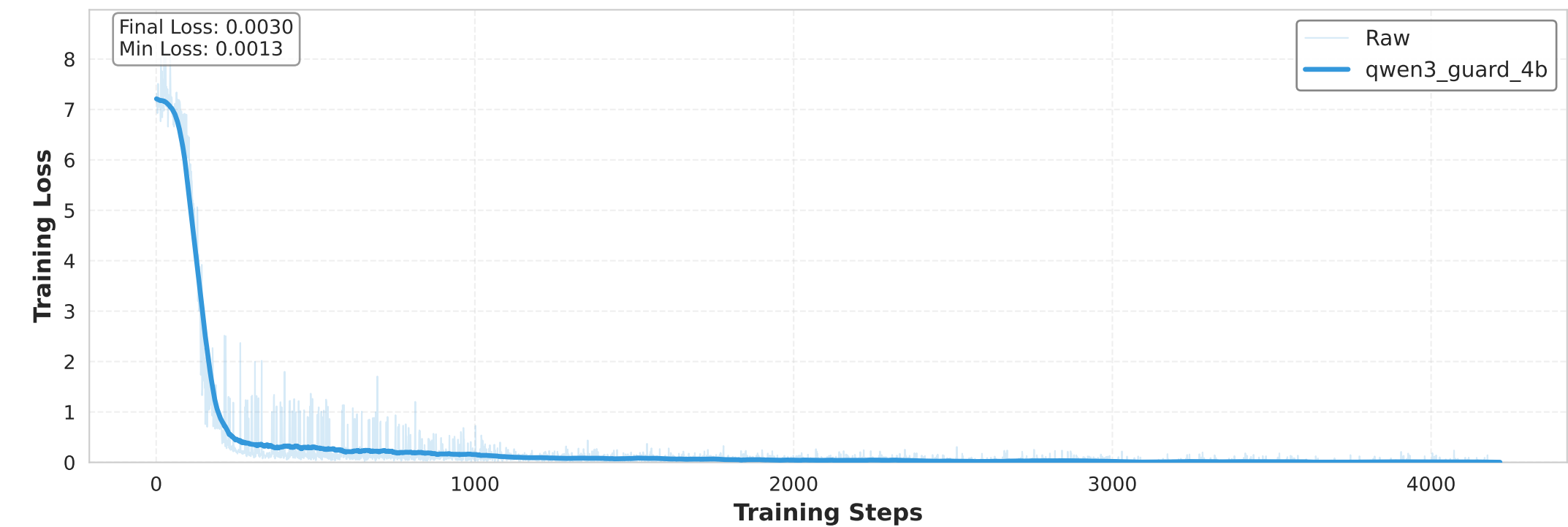
qwen3_guard_4b - Training Loss Curve
