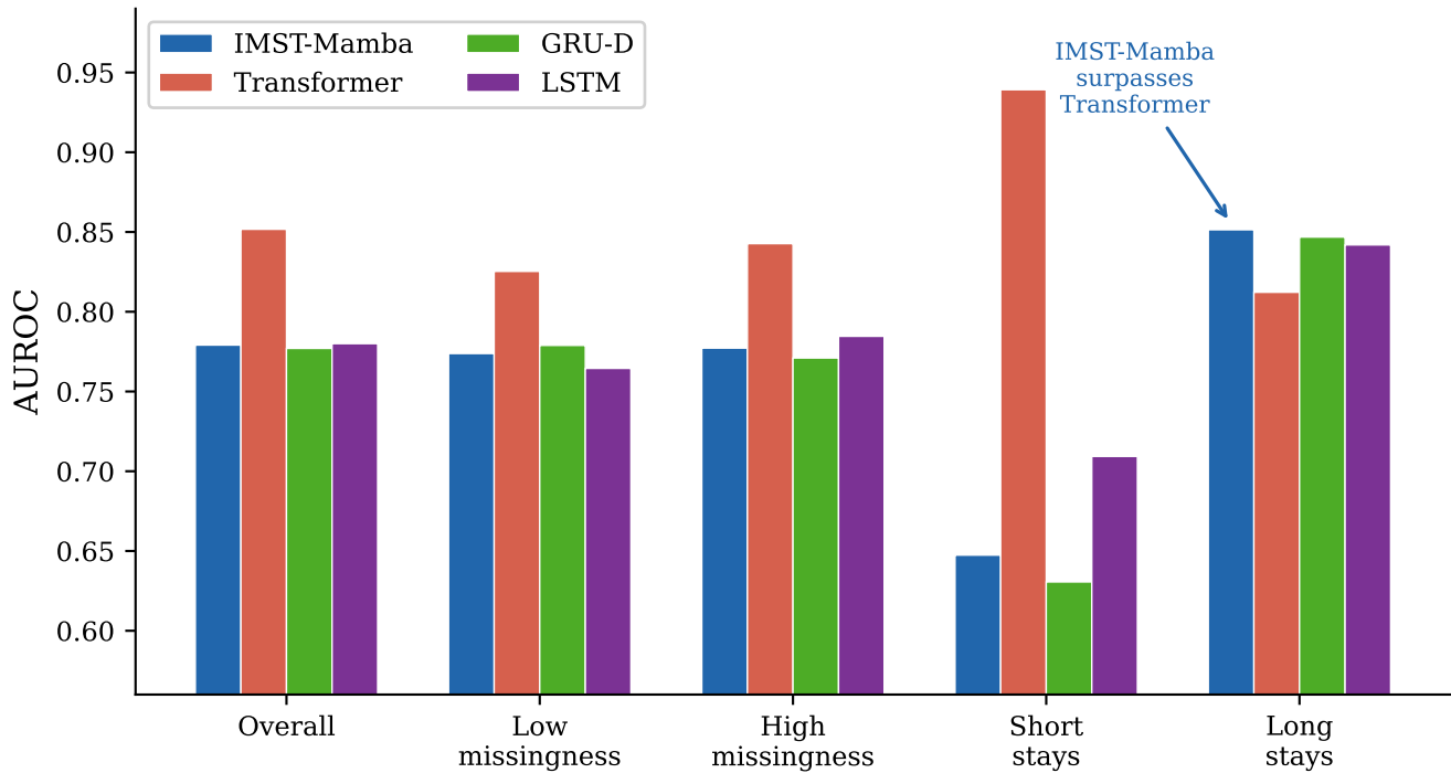
AUROC by Patient Subgroup
