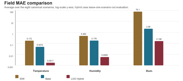
Fig. 4. Average field MAE for IDW, the base estimator, and leave-one-scenario-out hybrid residual correction. The y-axis is logarithmic.
