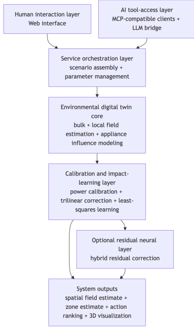
Fig. 1. Layered architecture of the proposed single-room spatial digital twin.
