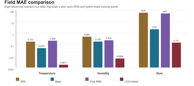
Fig. 4. Average field MAE for IDW, the base estimator, a pure RNN, and leave-one-scenario-out hybrid residual correction. The y-axis is logarithmic.
