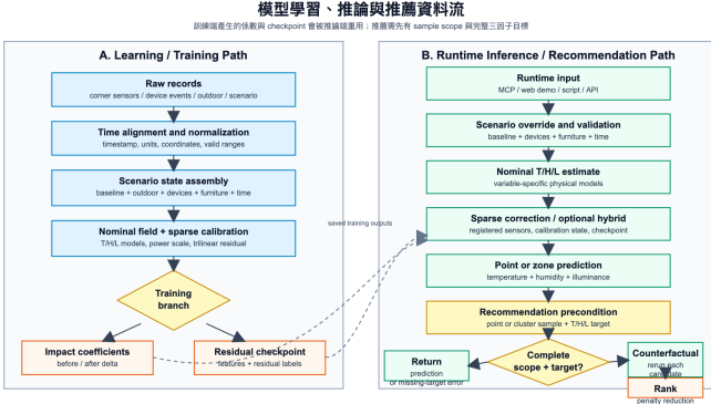
Fig. 3. Shared learning, inference, and recommendation data flow. Learned impact coefficients and the optional residual checkpoint are saved from the training path and reused by the runtime estimator.
