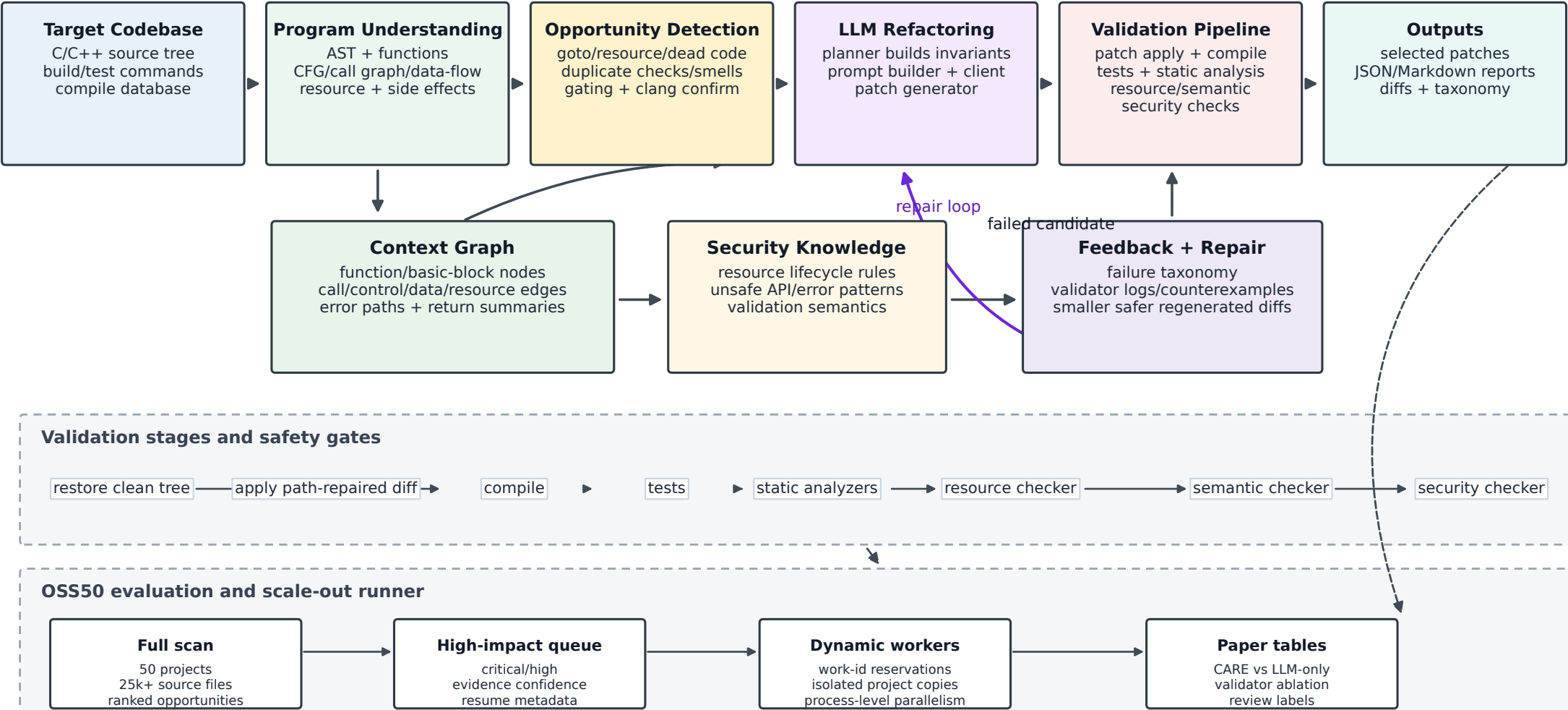
Figure: CARE integrates static program context with LLM patch generation and multi-stage validation; failed candidates feed back into repair.
