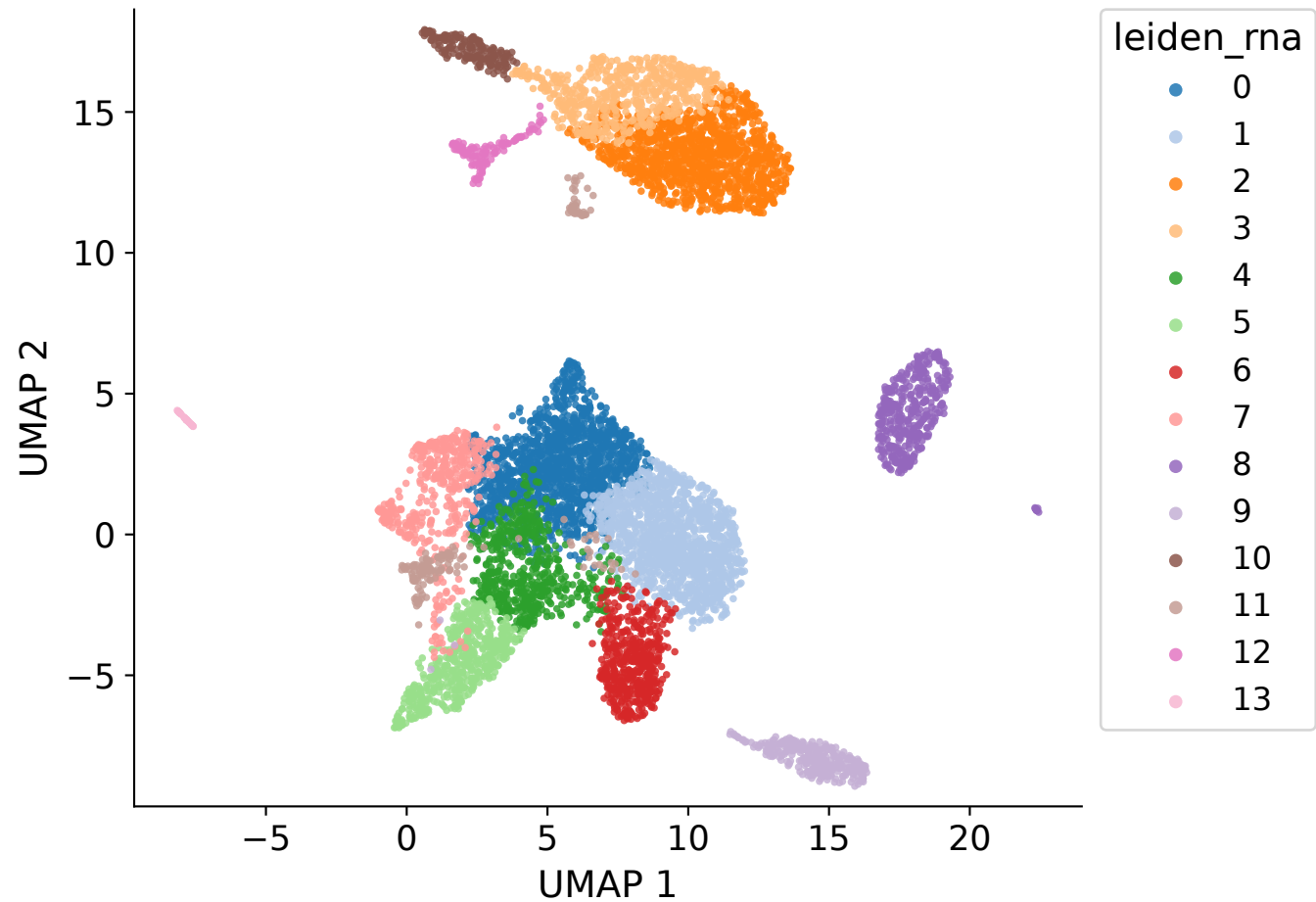
RNA UMAP — Leiden clusters
