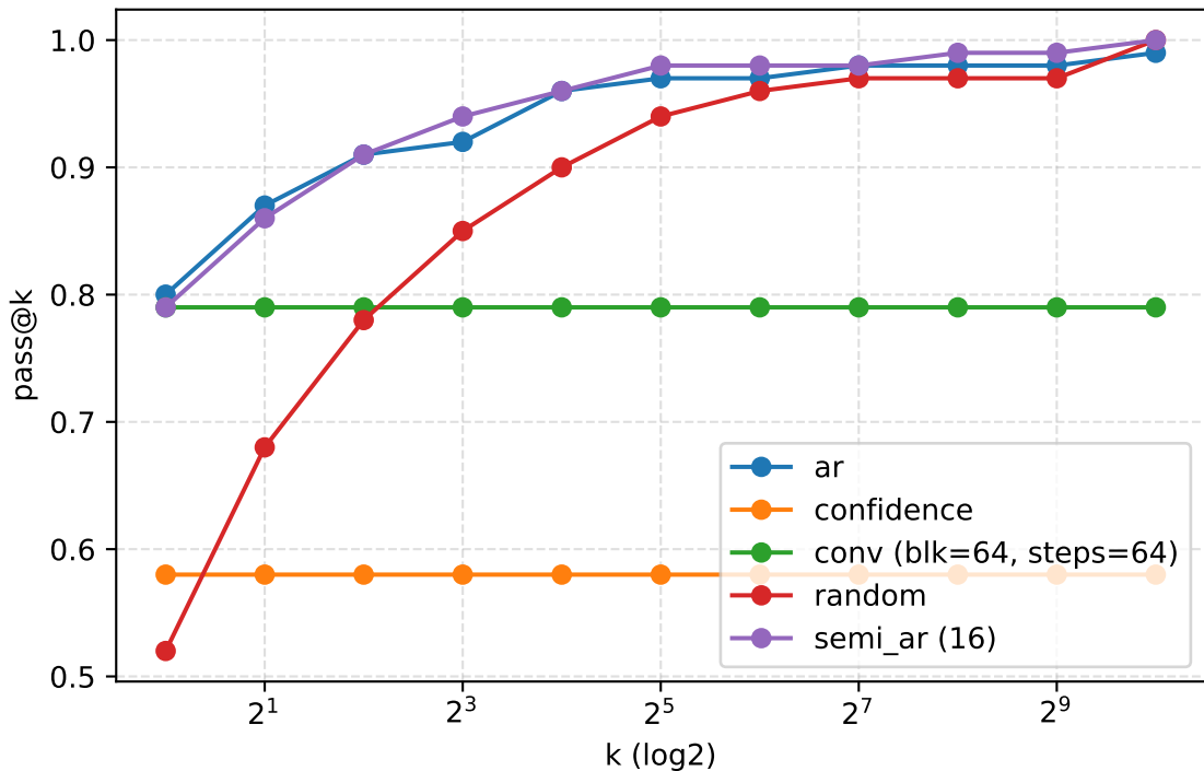
GSM8K pass@k by decoding method
