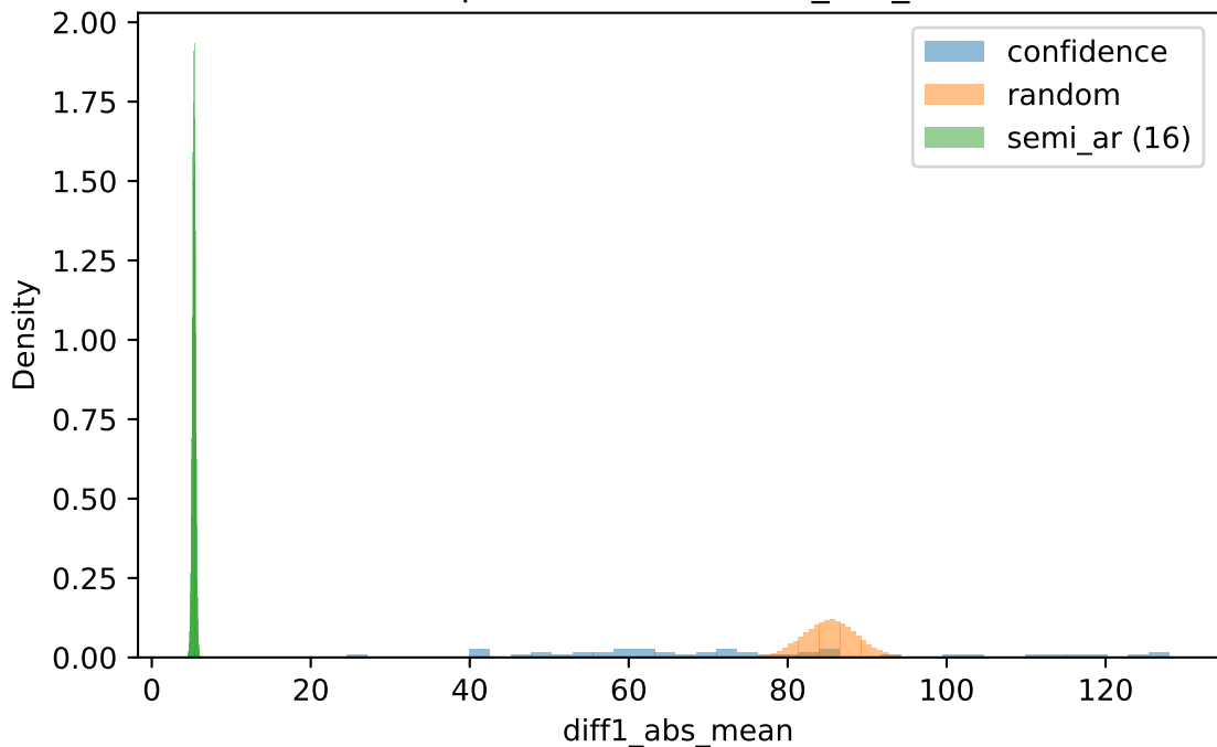
Failed permutations - diff1_abs_mean
