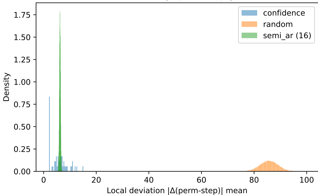
Local deviation |\Delta(\text{perm-step})| mean
