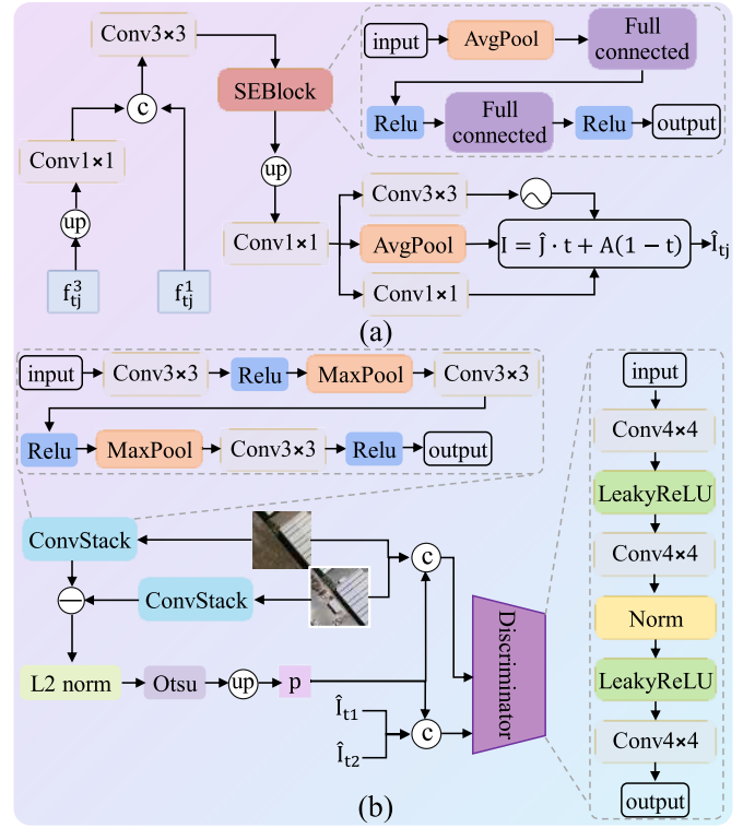
Fig. 5. (a) Illustration of the PGARM. (b) Illustration of the adversarial framework.
