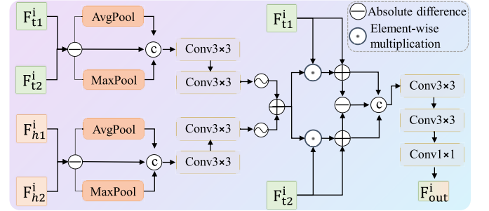
Fig. 4. Illustration of the HED module.
