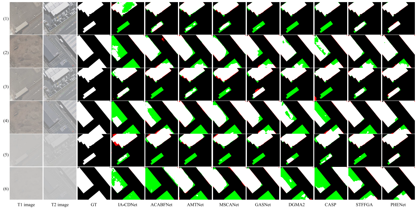
Fig. 6. Visual comparison of change detection results on WHU-CD dataset across fog densities. Rows (1) and (2), (3) and (4), and (5) and (6) show samples under light, medium, and heavy fog, respectively.
