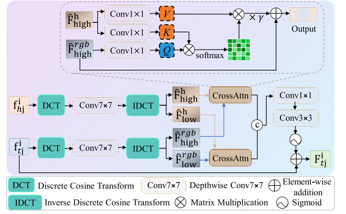
Fig. 3. Illustration of the HAMF module.
