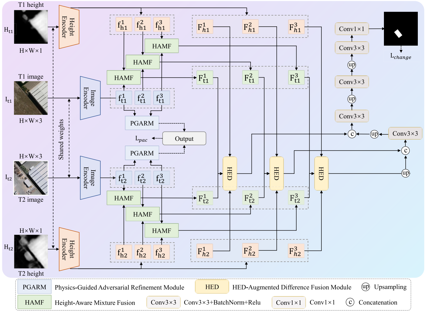
Fig. 1. Overview of the proposed PHENet framework.
