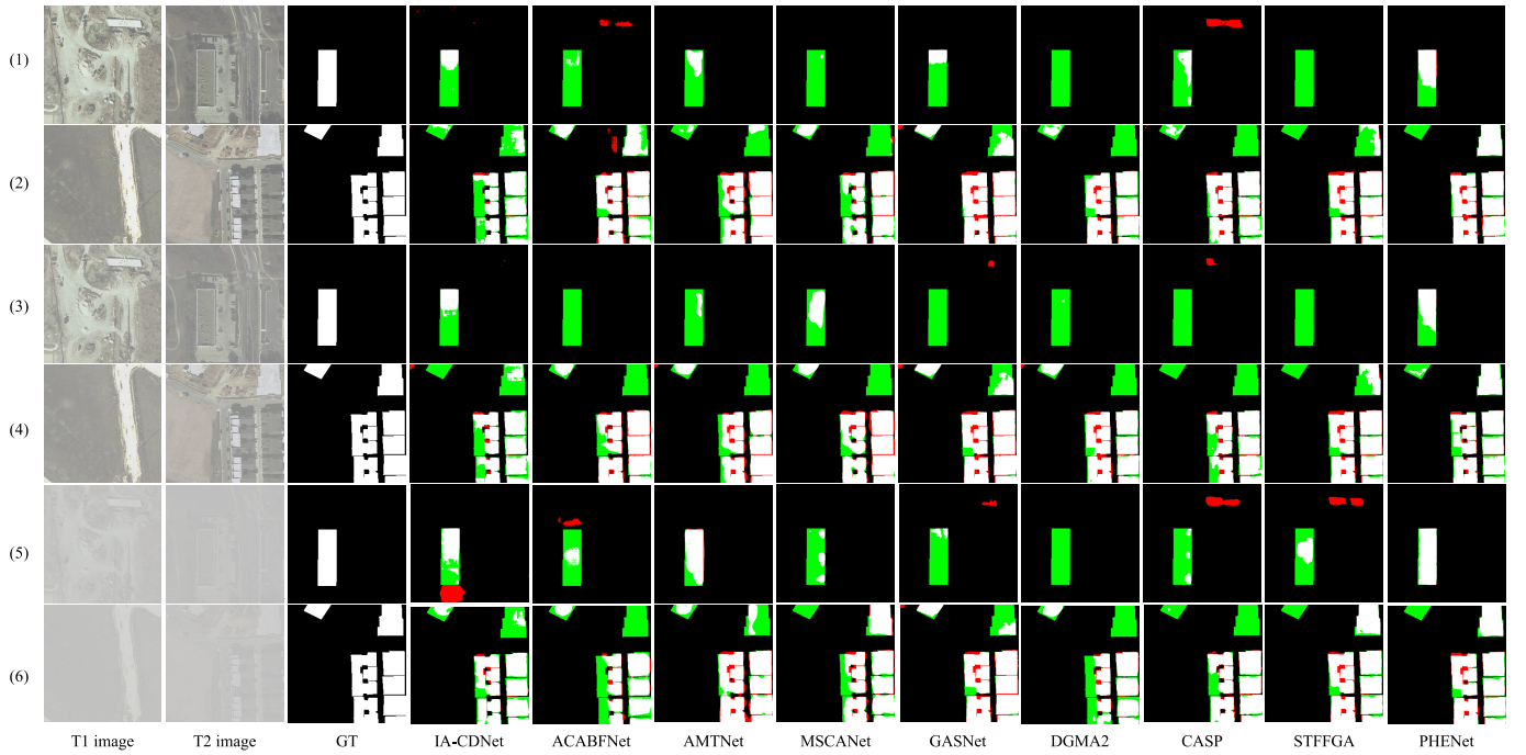
Fig. 7. Visual comparison of change detection results on LEVIR-CD dataset across fog densities. Rows (1) and (2), (3) and (4), and (5) and (6) show samples under light, medium, and heavy fog, respectively.
