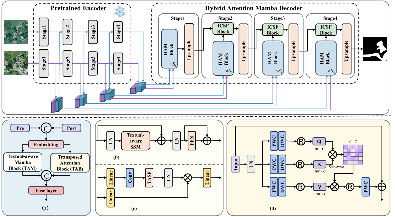
Fig. 2. Overall network architecture of our hybrid attention Mamba (HAM-CD) method. It comprises a weight-sharing Siamese encoder (VMamba-based) and a Mamba-based decoder with HAM blocks. The encoder extracts multitemporal features, while the decoder enhances spatial relationship learning through global–local feature interaction. The ICSF block adaptively fuses cross-stage features to enhance robust spatial–temporal feature representation. (a) HAM. (b) TAM block. (c) Textual-aware SSM. (d) TAB.
