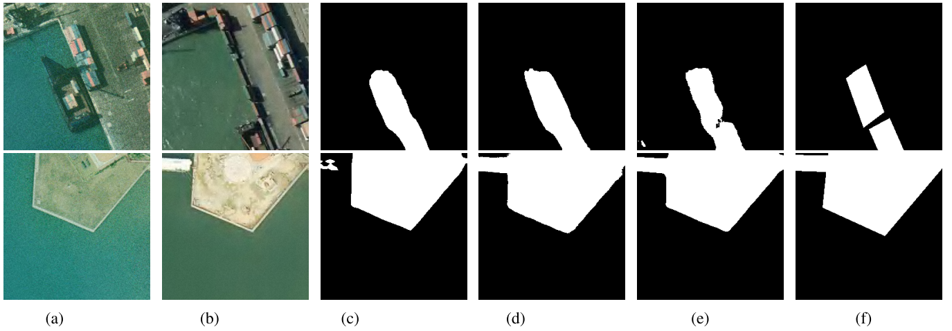
Fig. 7. Visualization of the change maps detected under water bodies interference on the SYSU-CD dataset. (a) Preetime. (b) Posttime. (c) ChangeFormer. (d) MambaBCD. (e) Ours. (f) GT.
