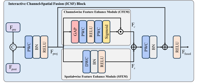
Fig. 3. Structure of the ICSF block. It adaptively fuses cross-stage features, enhancing robust spatial-temporal feature representation by jointly modeling their semantic differences in both channel- and spatial-wise dimensions.
