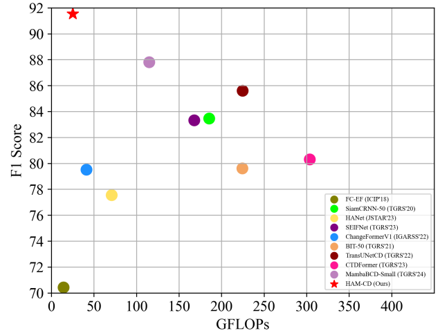
Fig. 1. Tradeoff between computational efficiency and CD performance. As shown, our HAM-CD strikes an optimal balance between performance and inference efficiency.
