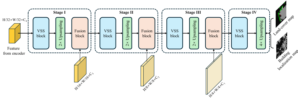
Fig. 6. Specific structure of the semantic decoder in MambaSCD and MambaBDA architectures.
