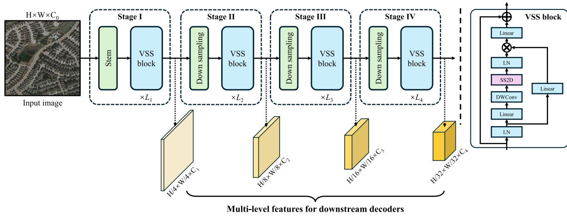
Fig. 2. Specific structure of the encoder network is based on the visual SSM used in our three architectures.
