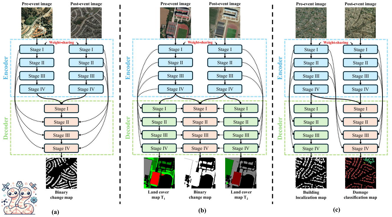
Fig. 1. Network framework of the proposed (a) MambaBCD for BCD, (b) MambaSCD for SCD, and (c) MamabBDA for BDA. The specific structure of the encoder and decoder is shown in Figs. 2, 4, and 6.
