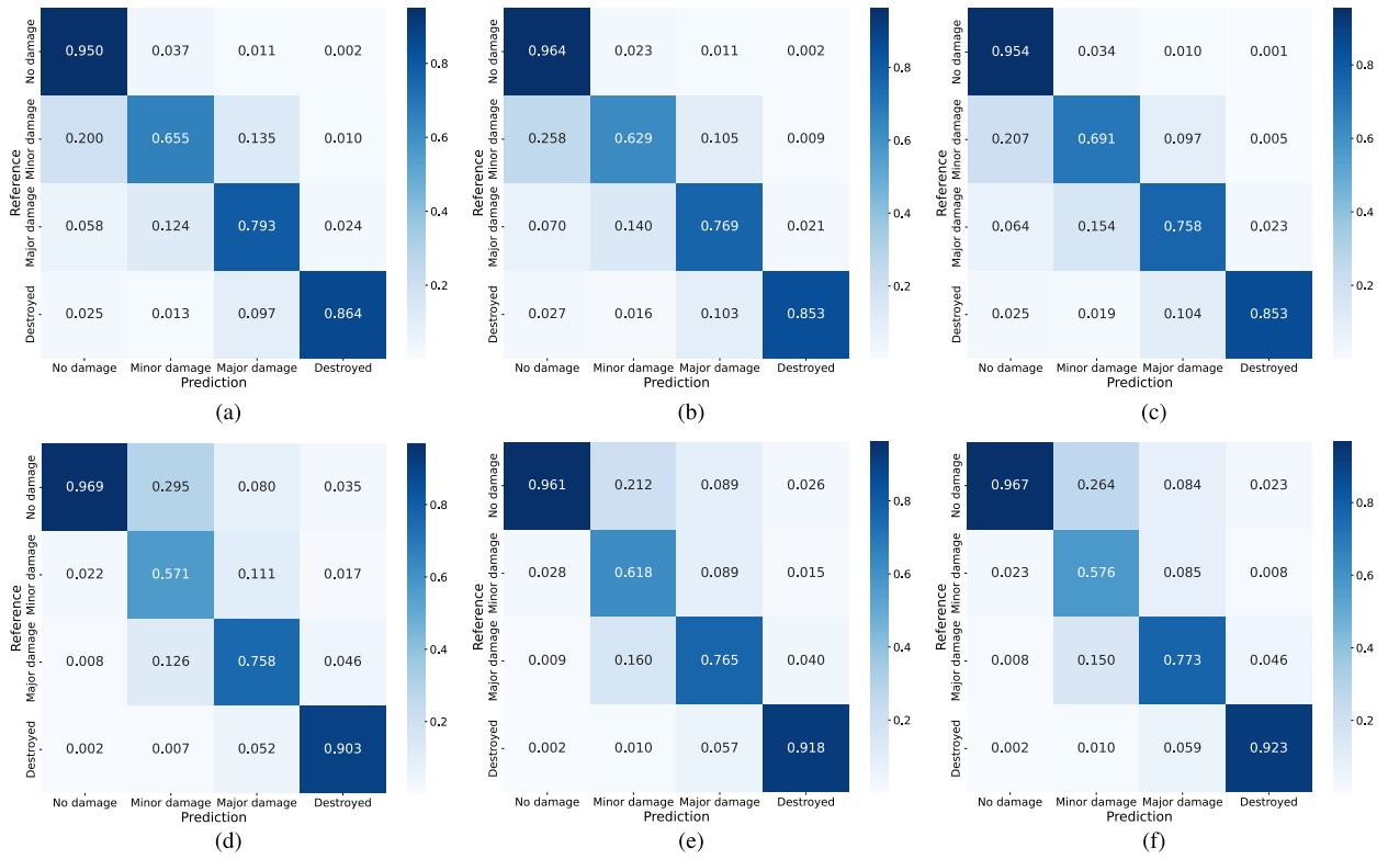
Fig. 10. Confusion matrices of MambaBDA-Tiny, MambaBDA-Small, and MambaBDA-Base. (a)–(c) Matrices normalized by rows. (d)–(f) Matrices normalized by columns.
