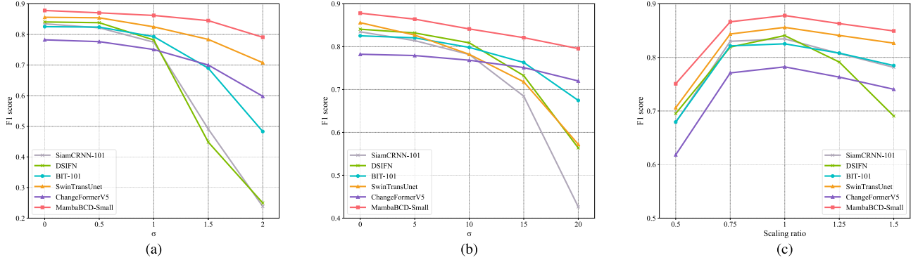
Fig. 14. Robustness of different models against degraded data on the LEVIR-CD+ dataset. (a) Gaussian blur. (b) Gaussian noise. (c) Scaling.
