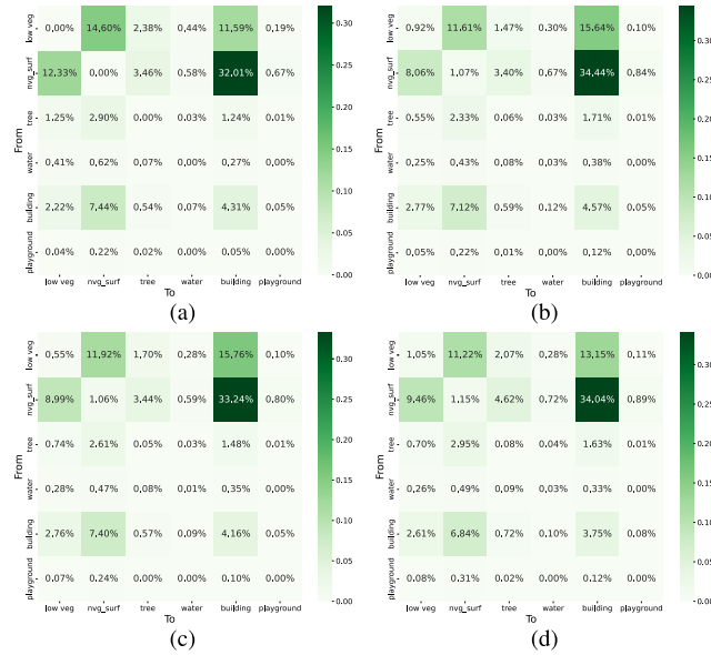
Fig. 8. Semantic change matrices providing “from-to” transition information derived from the SCD results. (a) Reference. (b) MambaSCD-Tiny. (c) MambaSCD-Small. (d) MambaSCD-Base.
