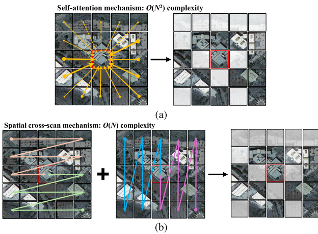
Fig. 3. Illustration of the (a) self-attention mechanism [29], [61] and (b) cross-scan mechanism [39] to capture global contextual information.
