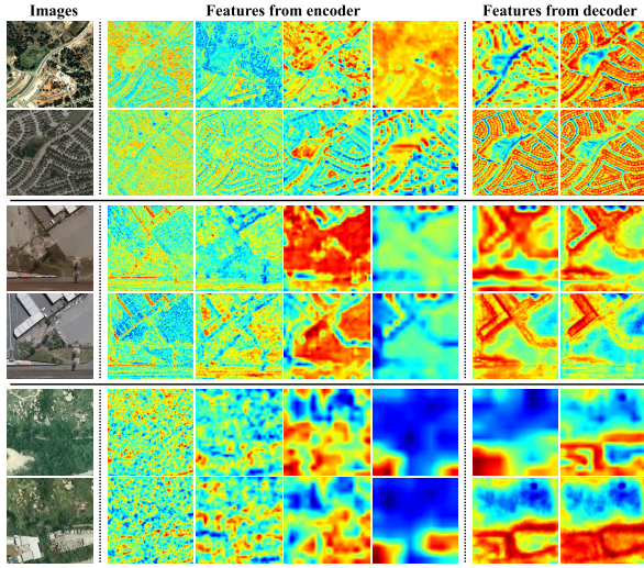
Fig. 12. Visualization of features from different layers of MambaBCD.
