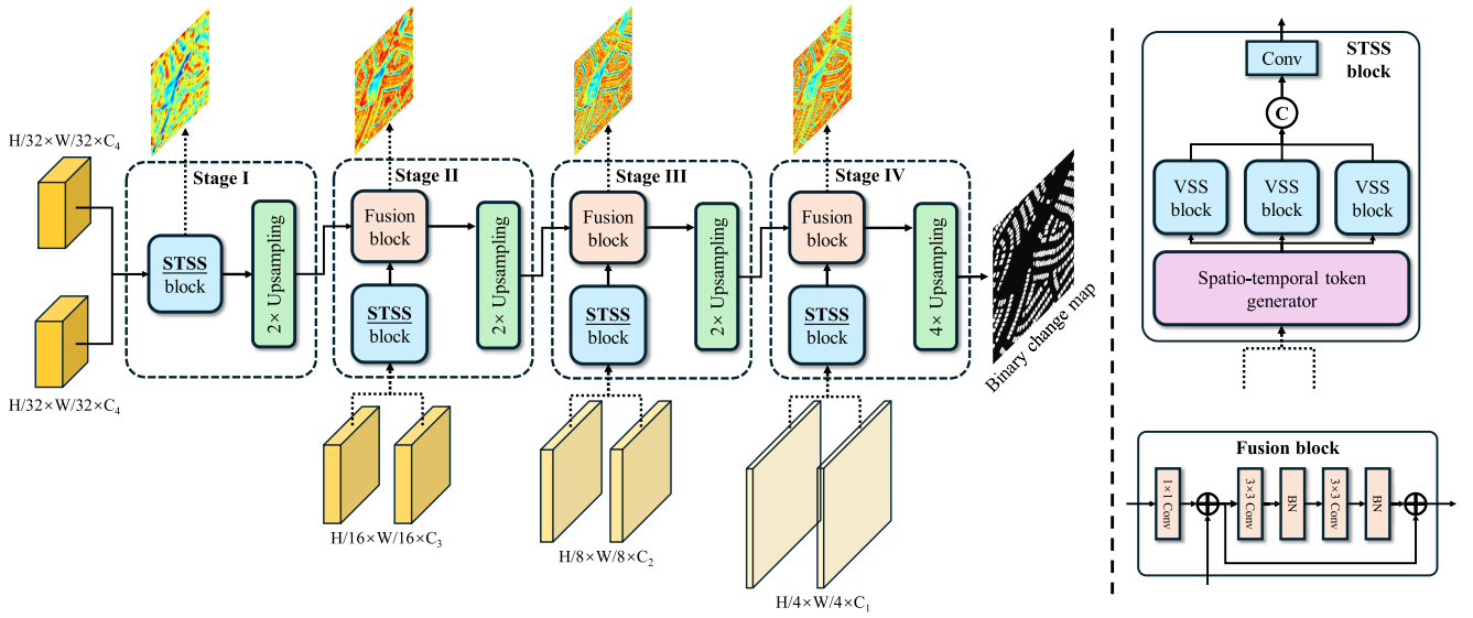
Fig. 4. Specific structure of the change decoder used in MambaBCD, MambaSCD, and MambaBDA architectures based on the proposed spatiotemporal relationship modeling mechanisms in Fig. 5.
