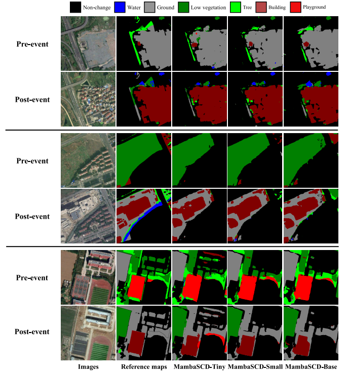
Fig. 9. Some semantic change maps obtained by the proposed MamabaSCD architectures on the test set of the SECOND dataset.
