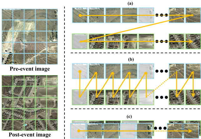
Fig. 5. Illustration of three mechanisms for learning spatiotemporal relationships. (a) Spatiotemporal sequential modelling. (b) Spatiotemporal cross modelling. (c) Spatiotemporal parallel modelling.
