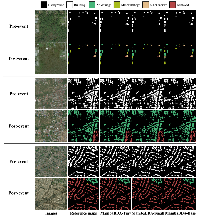
Fig. 11. Some BDA results obtained by our methods on the test set of the xBD dataset. From top to bottom, the disaster events are typhoons, tsunamis, and wildfires.
