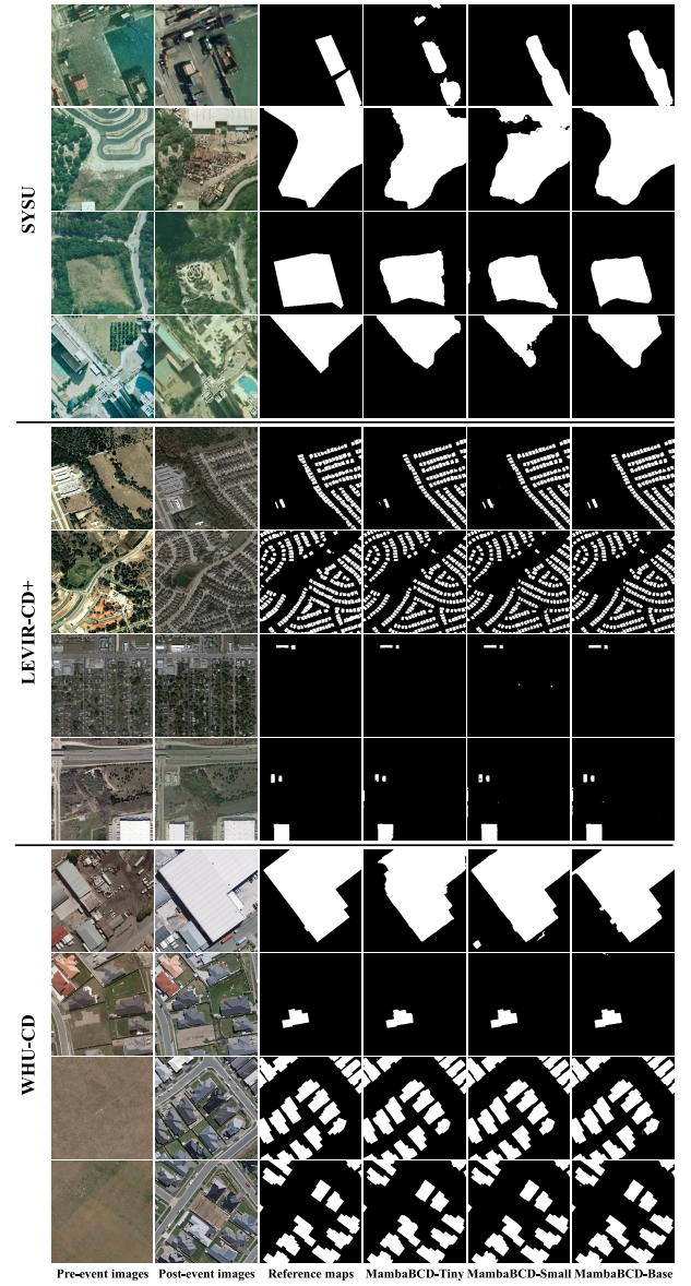
Fig. 7. Some binary change maps obtained by our methods on the test set of the three BCD dataset.
