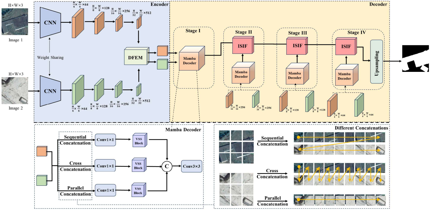
Fig. 1. Architecture of the proposed DEIF-Mamba.
