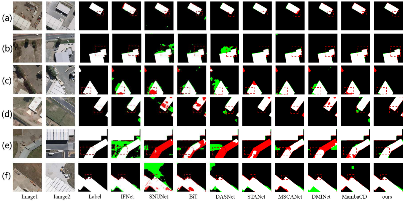
Fig. 7. Visual results of different models on test samples of WHU-CD. (a)–(f) Six representative samples.
