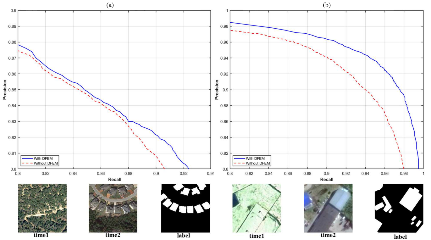
Fig. 8. Precision–recall curves on challenging cases in (a) LEVIR-CD and (b) CDD with and without DFEM.
