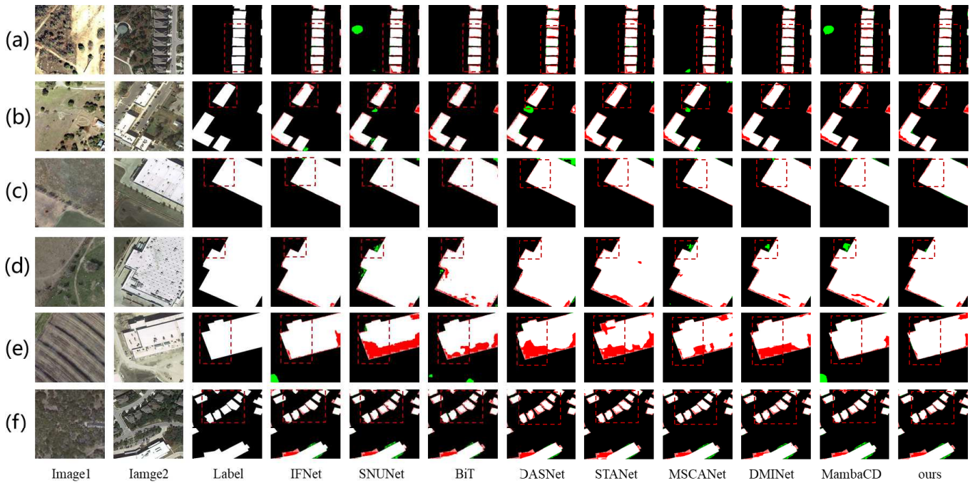
Fig. 4. Visual results of different models on test samples of LEVIR-CD. (a)–(f) Six representative samples.
