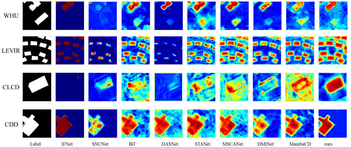
Fig. 10. Network visualization results of different models taking images from LEVIR-CD, CDD, CLCD, and WHU-CD as examples.
