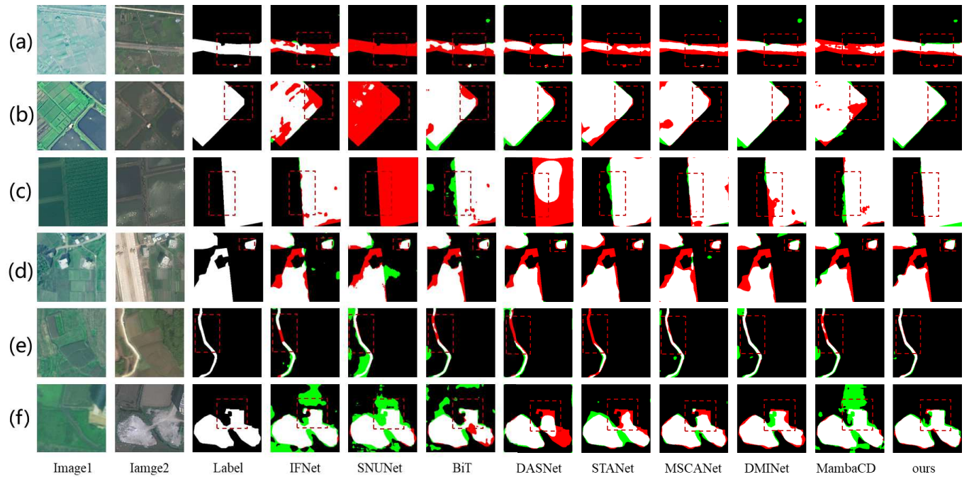
Fig. 6. Visual results of different models on test samples of CLCD. (a)–(f) Six representative samples.
