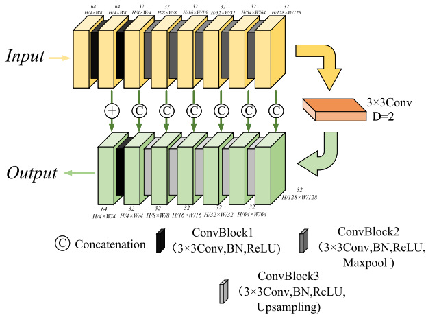
Fig. 5. Overview of residual U-block.
