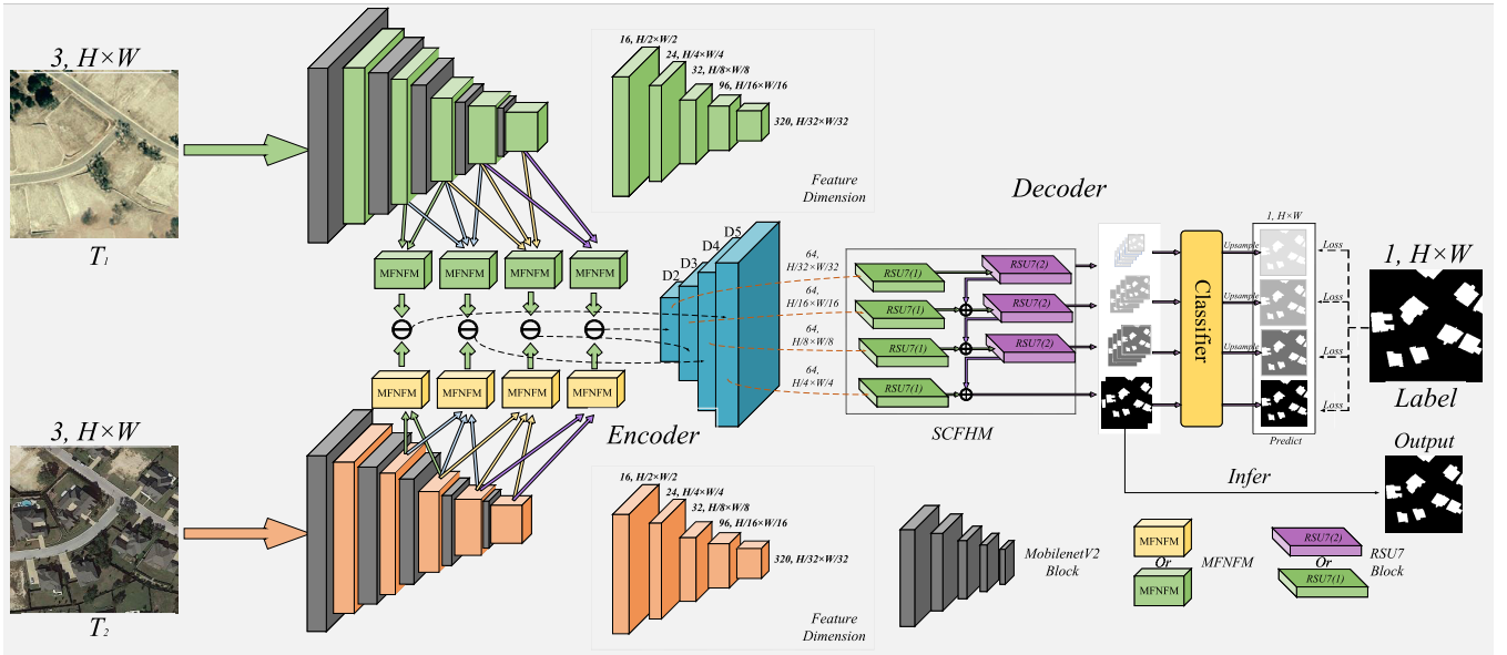
Fig. 3. Proposed EAFH-Net framework utilizes the MobileNetV2 network as the backbone in a Siamese-network configuration with weight sharing, to extract features of bi-temporal image pairs. Features from different scales are fed to the MFNFM module for the spatial information fusion of adjacent features. The output difference map undergoes spatial and channel feature information reconciliation through the SCFHM module, which consists of two stacked residual U-blocks-7 (RSU7) layers. This process further blends sophisticated and elementary-level features. Finally, scale alignment is performed through upsampling, yielding the change map as the output.
