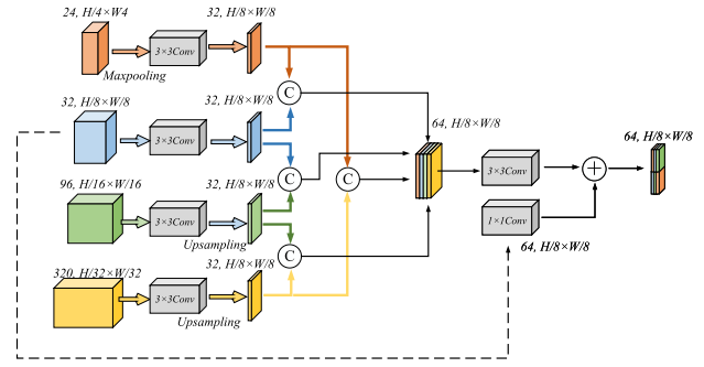
Fig. 13. Overview of MFNFM (all-feature fusion version).
