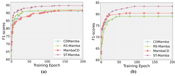
Fig. 5. Graphs show the changes in optimal F1 -scores on the test set during the training process for each experimental method. The line graph maintains the best-result node every 40 iterations to ensure continuity, even if no superior results are obtained subsequently. (a) Results on the WHU-CD dataset. (b) Results on the SYSU dataset.
