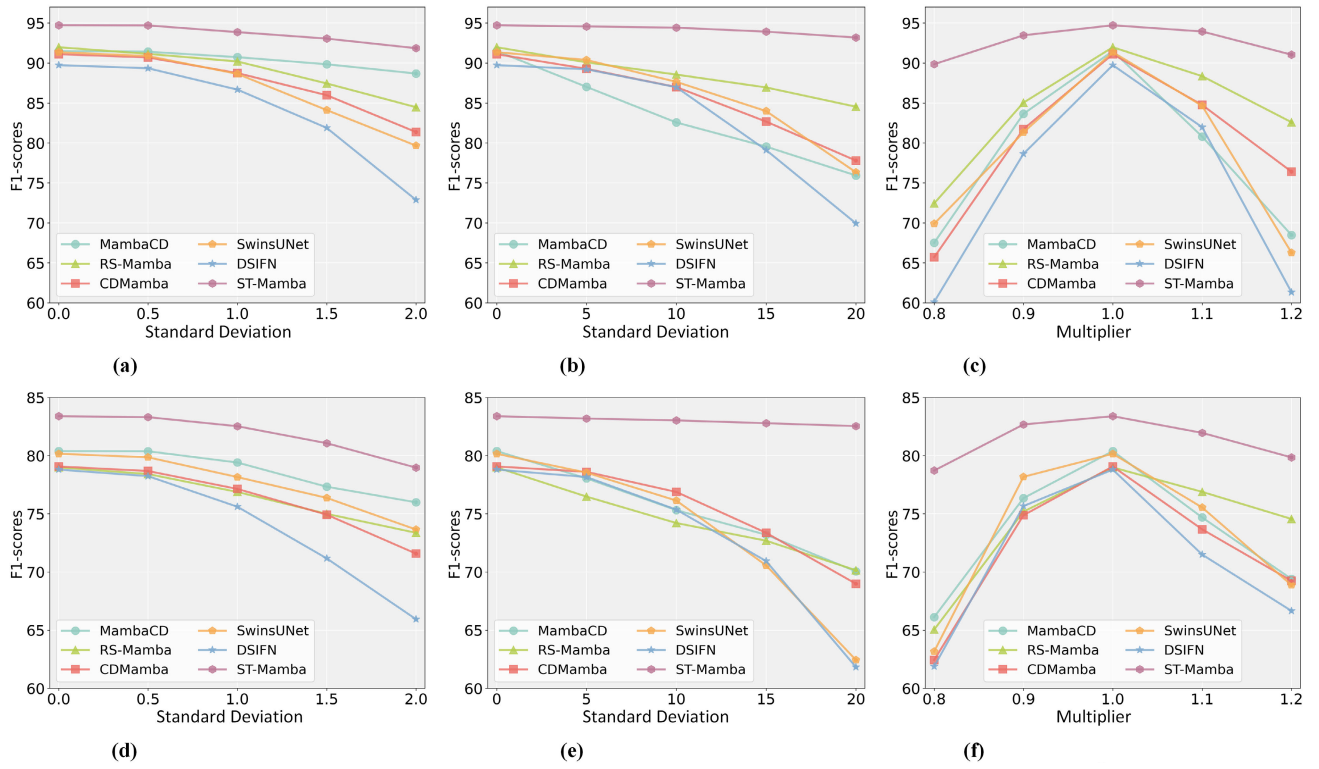
Fig. 11. Robustness of various models when tested against degraded images from the SYSU and WHU-CD datasets. (a) WHU GaussianBlur. (b) WHU GaussNoise. (c) WHU MultiplicativeNoise. (d) SYSC GaussianBlur. (e) SYSU GaussNoise. (f) SYSU MultiplicativeNoise.
