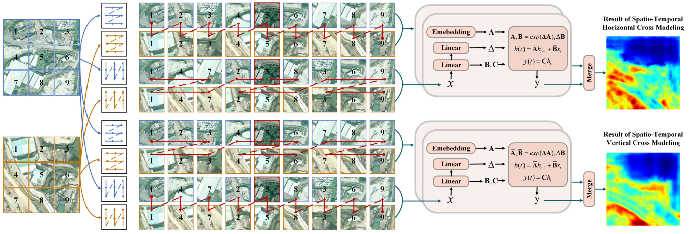
Fig. 4. Following two ST modeling processes in STSM are demonstrated: STHCM and STVCM. The blue color in the figure represents the feature information of pre-change images, and the yellow color represents the feature information of post-change images. In the schematic with blue and yellow arrows, the horizontal direction indicates horizontal scanning, and the vertical direction indicates vertical scanning. The red arrow represents the scanning direction used in the ST modeling process.
