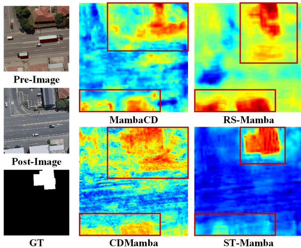
Fig. 8. Heatmap visualization of the feature maps for the WHU-CD dataset illustrates the probability of change for each pixel. Areas closer to red indicate a higher likelihood of change, while areas closer to blue suggest a greater probability of nonchange. The red boxes highlight the parts that are specifically compared in this article.
