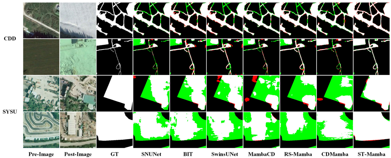
Fig. 7. Qualitative results on the CDD and SYSU datasets. Pre-images and post-images are images captured before and after the change, respectively. GT is the ground truth. In the result plots for each method, white indicates true positives, black indicates true negatives, green indicates false negatives, and red indicates false positives.
