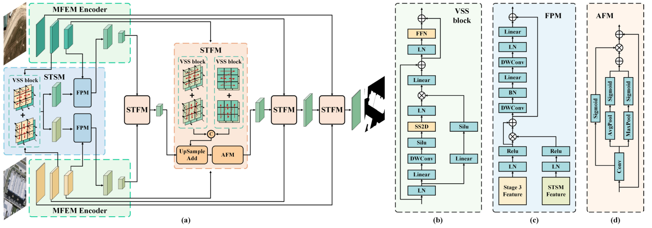
Fig. 2. Illustration of our method. (a) Overview of the ST-mamba framework. Given a pre-change and post-change image, the initial extraction of features is performed by the MFEM. These features are then fed into the STSM, where they are unified into a unified domain through a synergistic effect. Finally, the unified features are fed into a decoder consisting of STFM, which integrates multiscale and multichannel features to generate the final change map. (b) Schematic of the structure of the VSS blocks. (c) Structure schematic of the FPM in the STSM. (d) Structure schematic of the AFM in the STFM.
