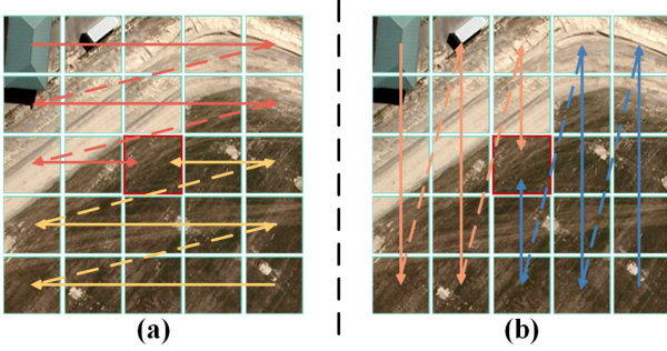
Fig. 3. Illustration of the cross-scan mechanism [26]. In this example, (a) horizontal cross-scan and (b) vertical cross-scan used to capture global contextual information.
