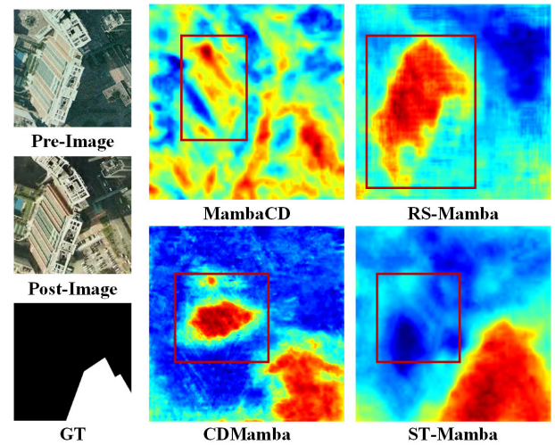
Fig. 9. Heatmap visualization of the feature maps for the SYSU dataset illustrates the probability of change for each pixel. Areas closer to red indicate a higher likelihood of change, while areas closer to blue suggest a greater probability of nonchange. The red boxes highlight the parts that are specifically compared in this article.
