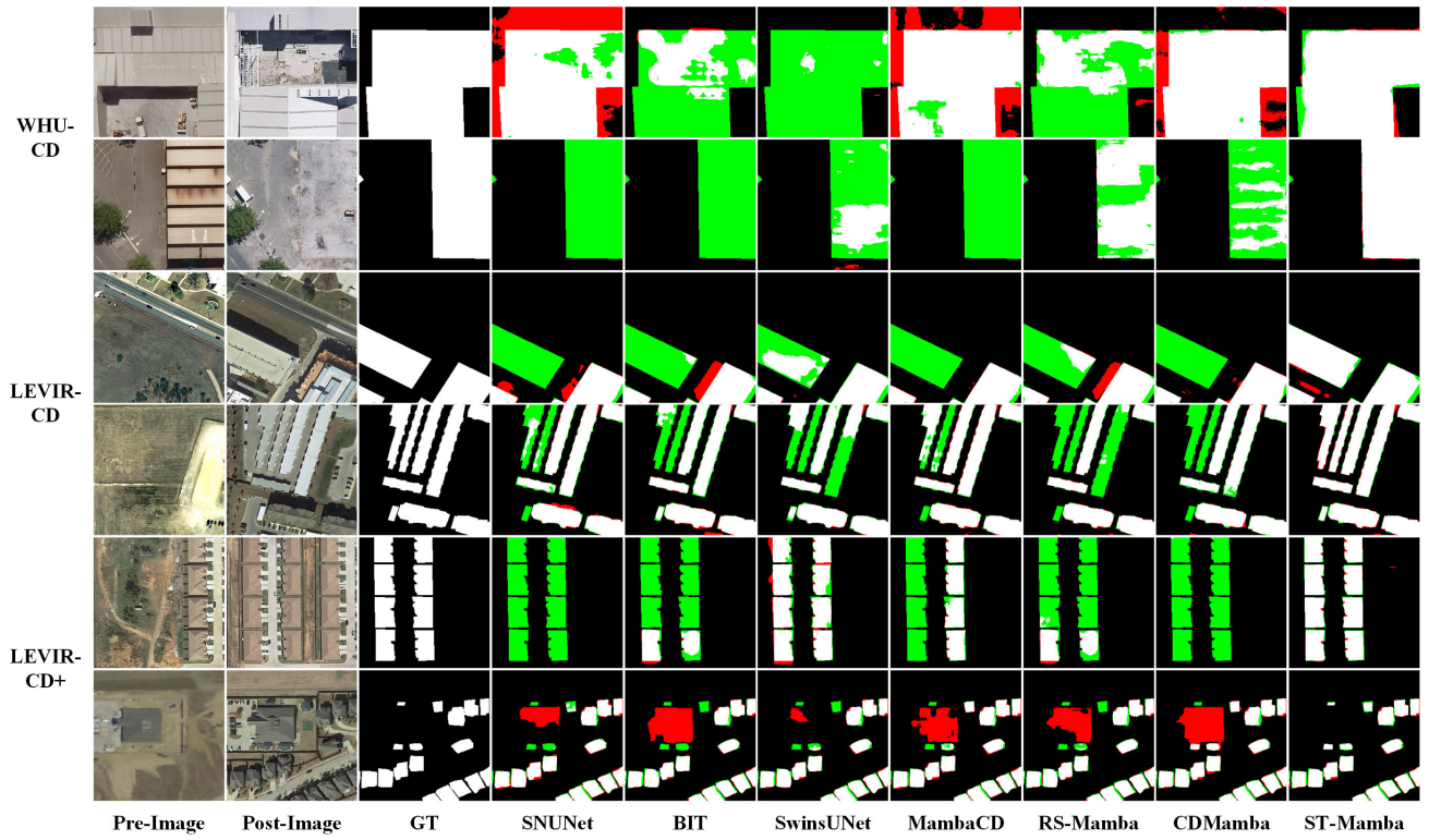
Fig. 6. Qualitative results on the WHU-CD, LEVIR-CD, and LEVIR-CD+ datasets. Pre-images and post-images are images captured before and after the change, respectively. GT denotes the ground truth. In the result plots for each method, white indicates true positives, black indicates true negatives, green indicates false negatives, and red indicates false positives.
