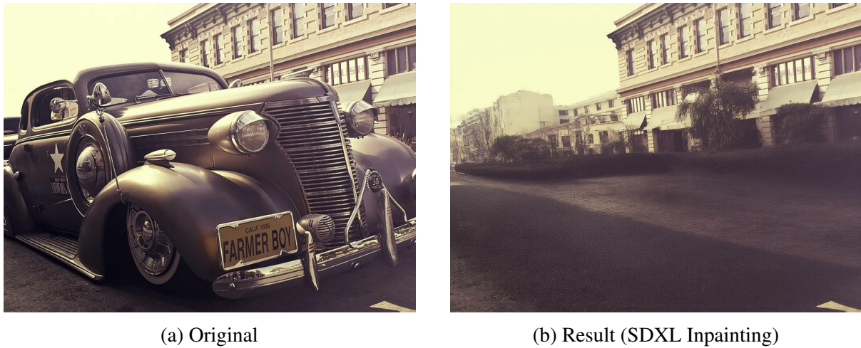
Figure 9: Inpainting result: removing a vintage car and generating an empty cobblestone road.
