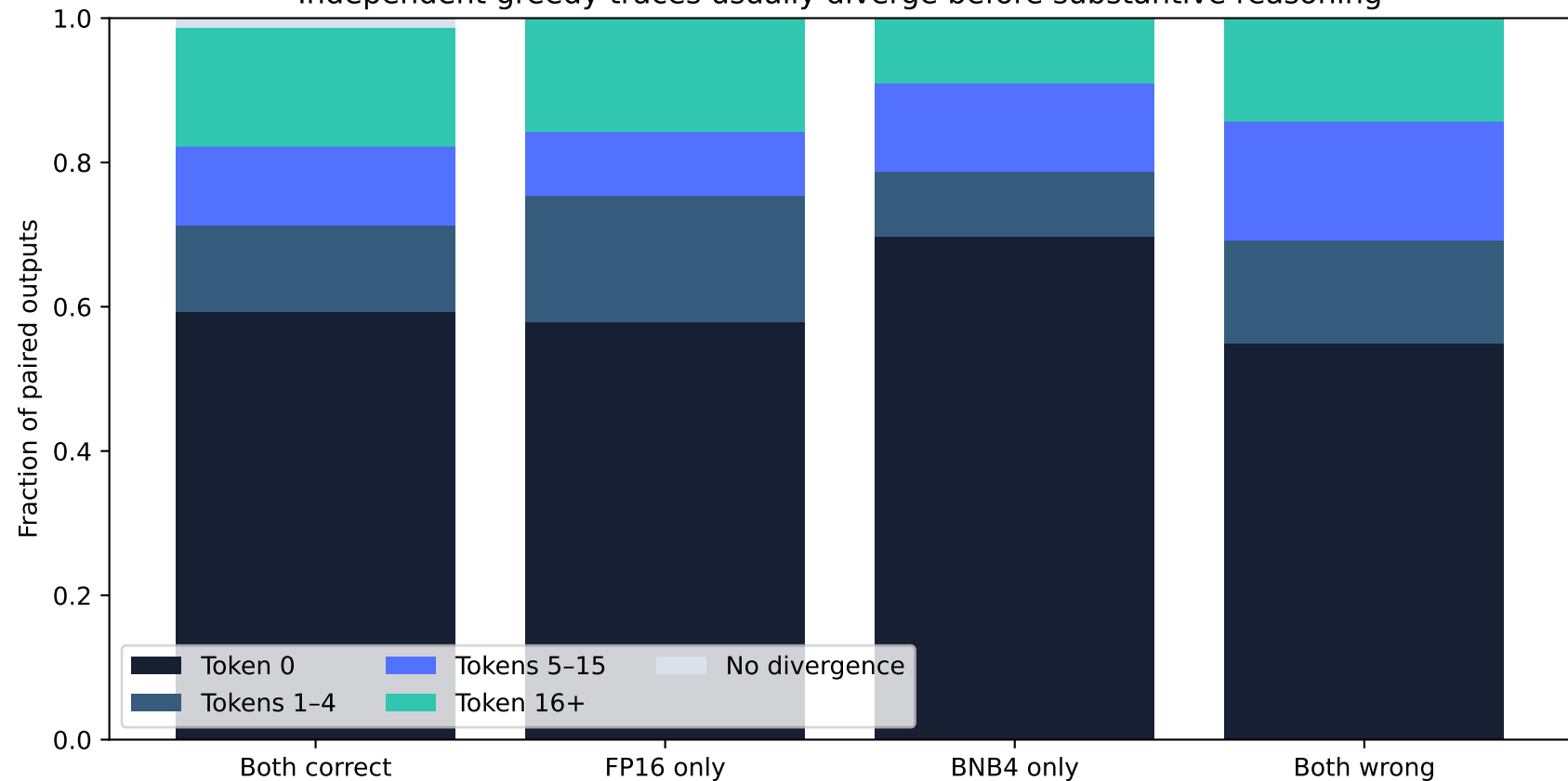
Independent greedy traces usually diverge before substantive reasoning
