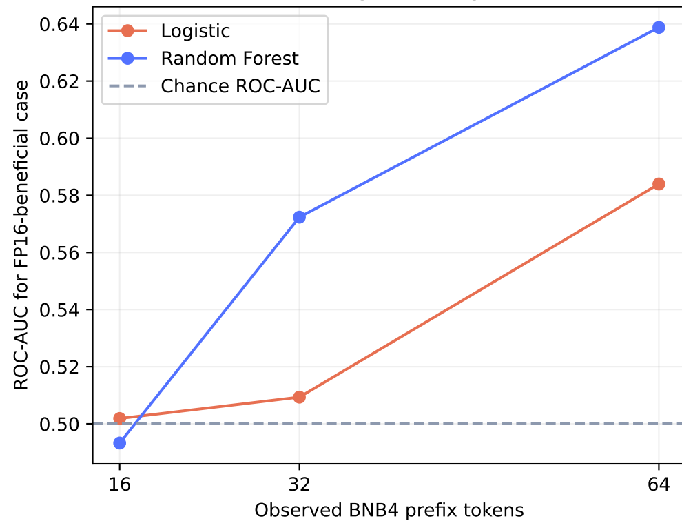
Predictive signal emerges late
