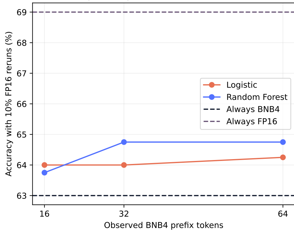
Early routing does not beat static FP16
