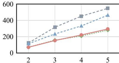
(c) HumanEval
