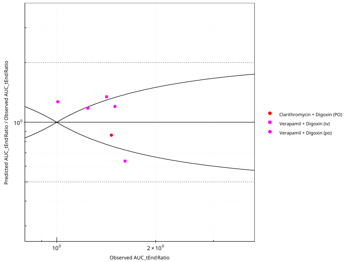
Figure 2-10: Pgp DDI. Mechanism: Mechanism-based Inactivation. Predicted/Observed vs. Observed AUC_tEnd Ratio. ( \delta = 1 in Guest et al. formula)
