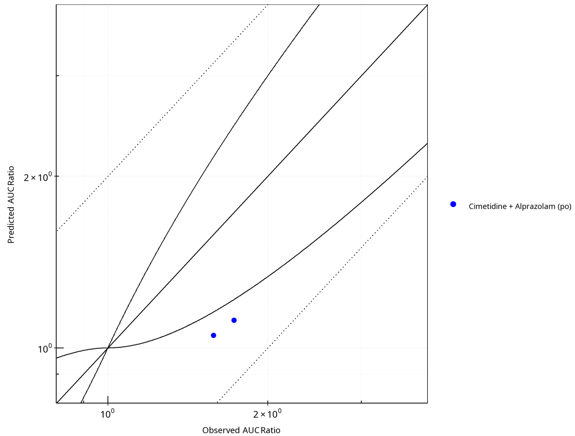
Figure 1-1: Plot. Predicted vs. Observed AUC Ratio. ( \delta = 1 in Guest et al. formula)
