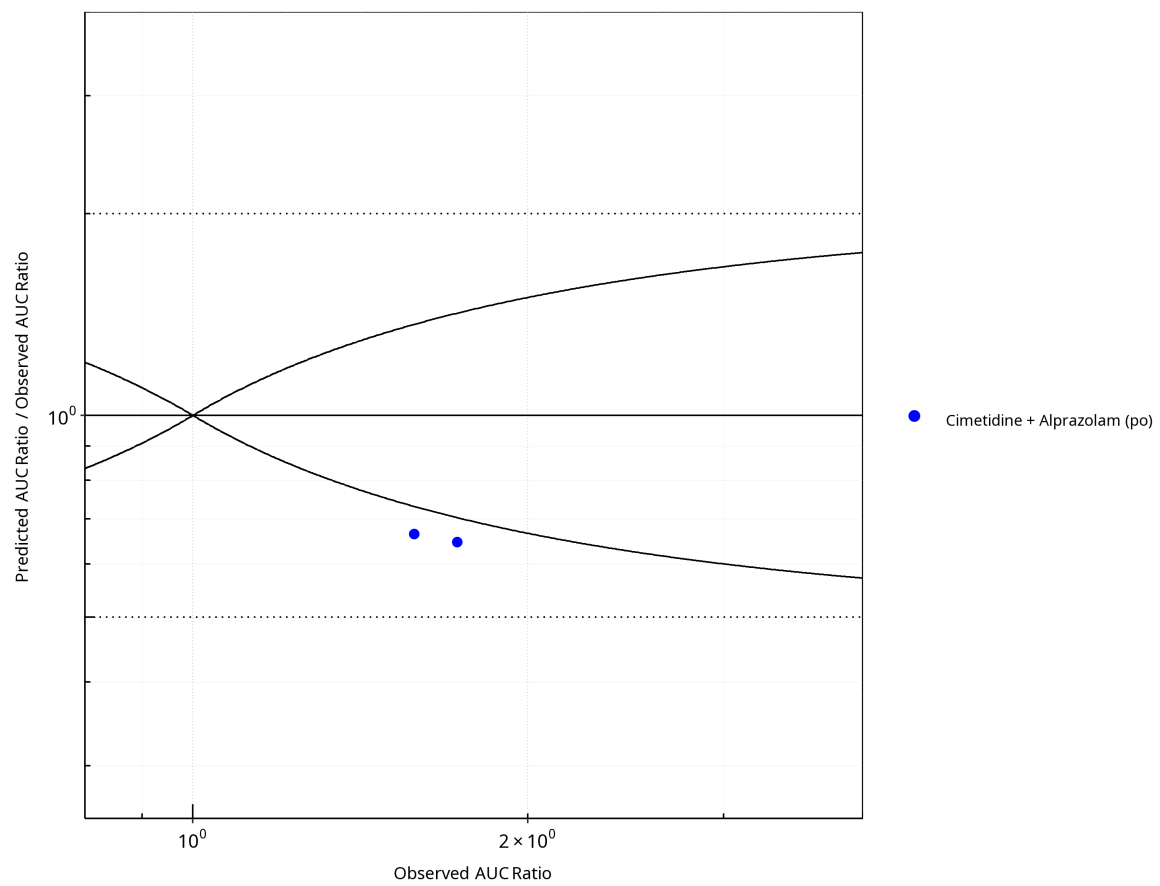
Figure 1-6: Plot. Mechanism: Reversible Inhibition. Predicted/Observed vs. Observed AUC Ratio. ( \delta = 1 in Guest et al. formula)
