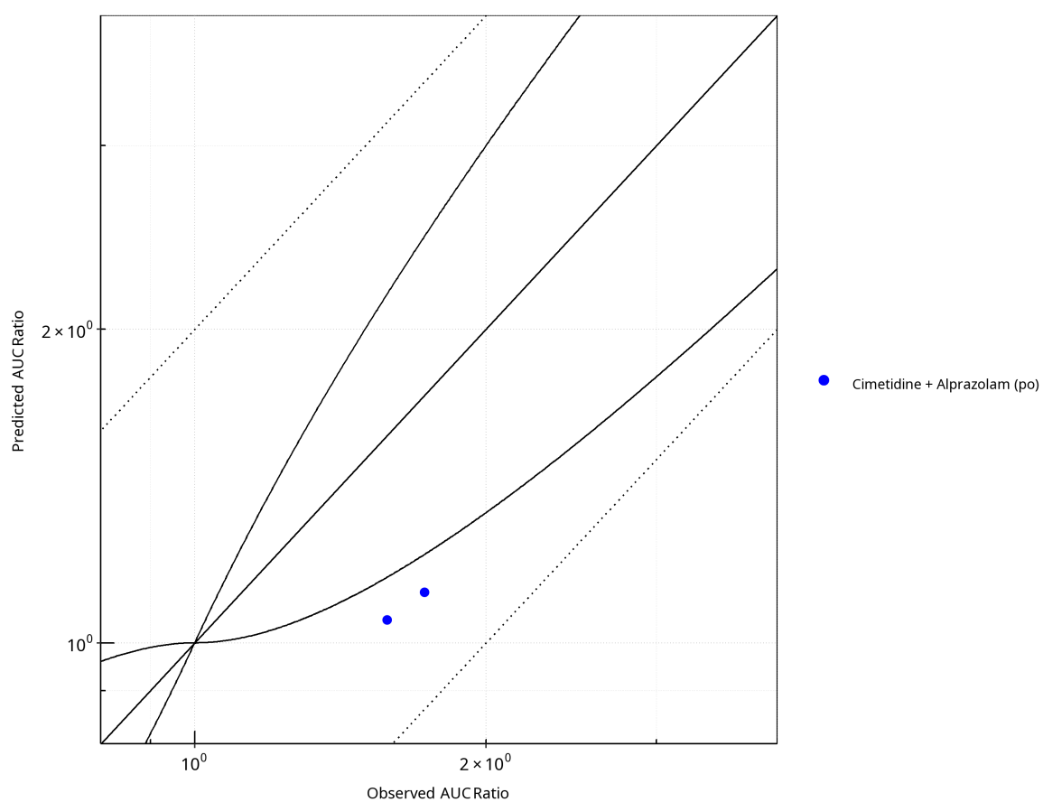
Figure 1-13: Plot. Victim: Alprazolam. Predicted vs. Observed AUC Ratio. ( \delta = 1 in Guest et al. formula)
