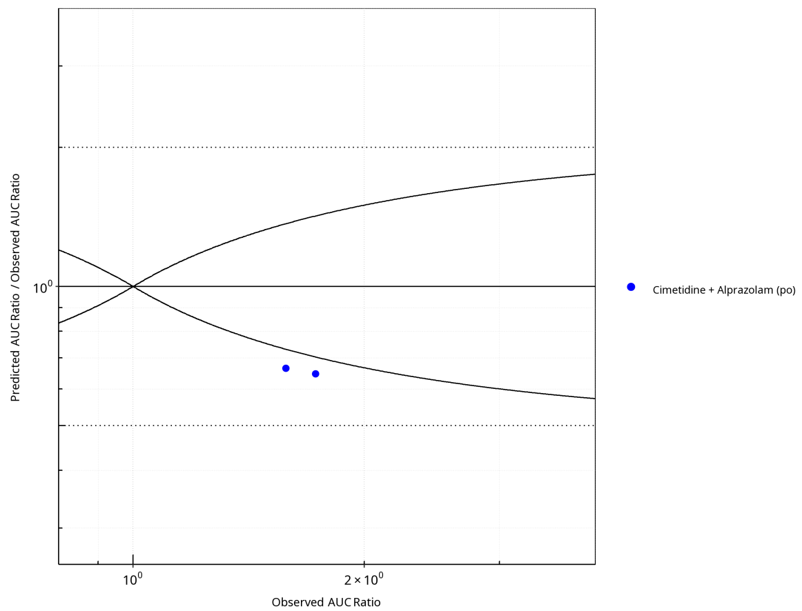
Figure 1-2: Plot. Predicted/Observed vs. Observed AUC Ratio. ( \delta = 1 in Guest et al. formula)
