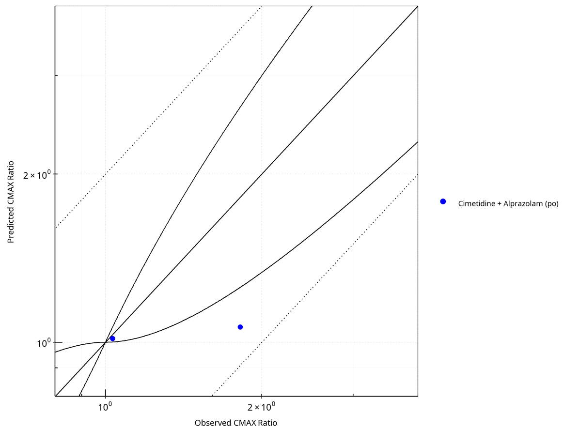
Figure 1-3: Plot. Predicted vs. Observed CMAX Ratio. ( \delta = 1 in Guest et al. formula)
