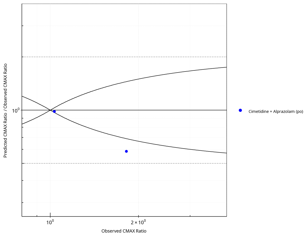
Figure 1-12: Plot. Perpetrator: Cimetidine. Predicted/Observed vs. Observed CMAX Ratio. ( \delta = 1 in Guest et al. formula)
