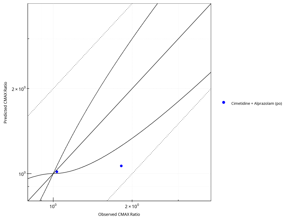
Figure 1-15: Plot. Victim: Alprazolam. Predicted vs. Observed CMAX Ratio. ( \delta = 1 in Guest et al. formula)
