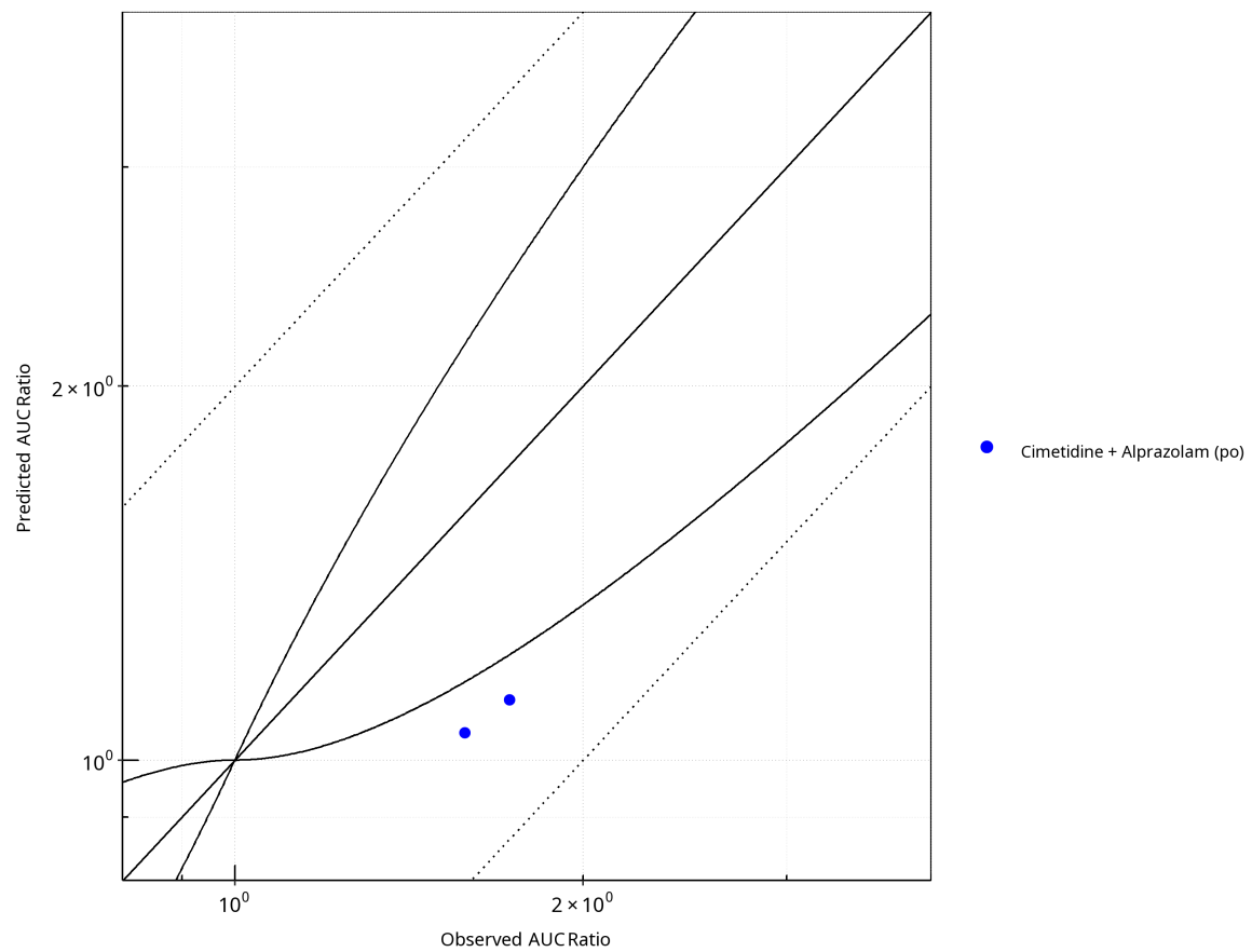
Figure 1-1: Plot. Predicted vs. Observed AUC Ratio. ( \delta = 1 in Guest et al. formula)
