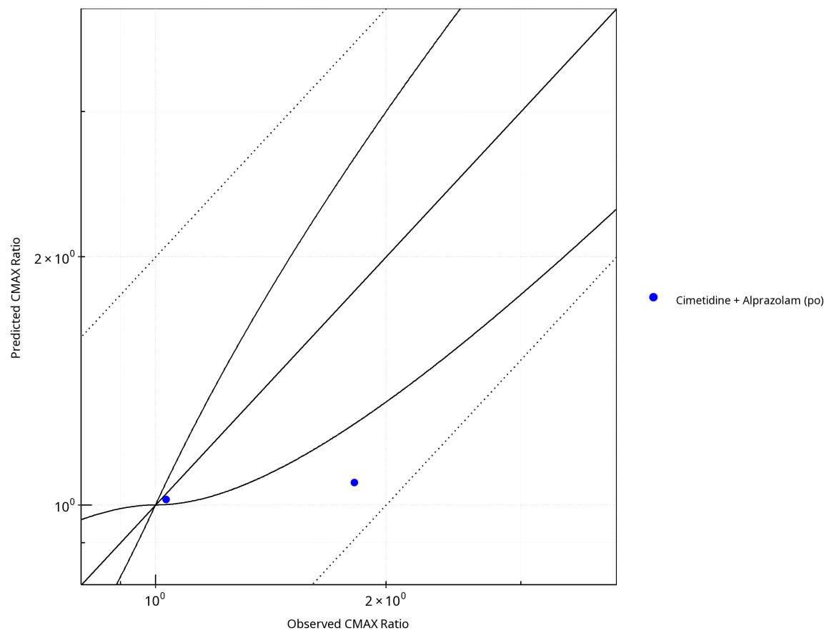
Figure 1-7: Plot. Mechanism: Reversible Inhibition. Predicted vs. Observed CMAX Ratio. ( \delta = 1 in Guest et al. formula)
