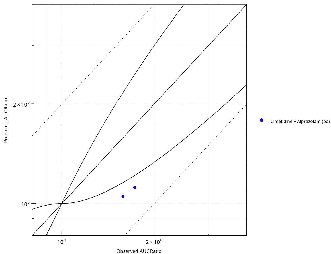
Figure 1-9: Plot. Perpetrator: Cimetidine. Predicted vs. Observed AUC Ratio. ( \delta = 1 in Guest et al. formula)
