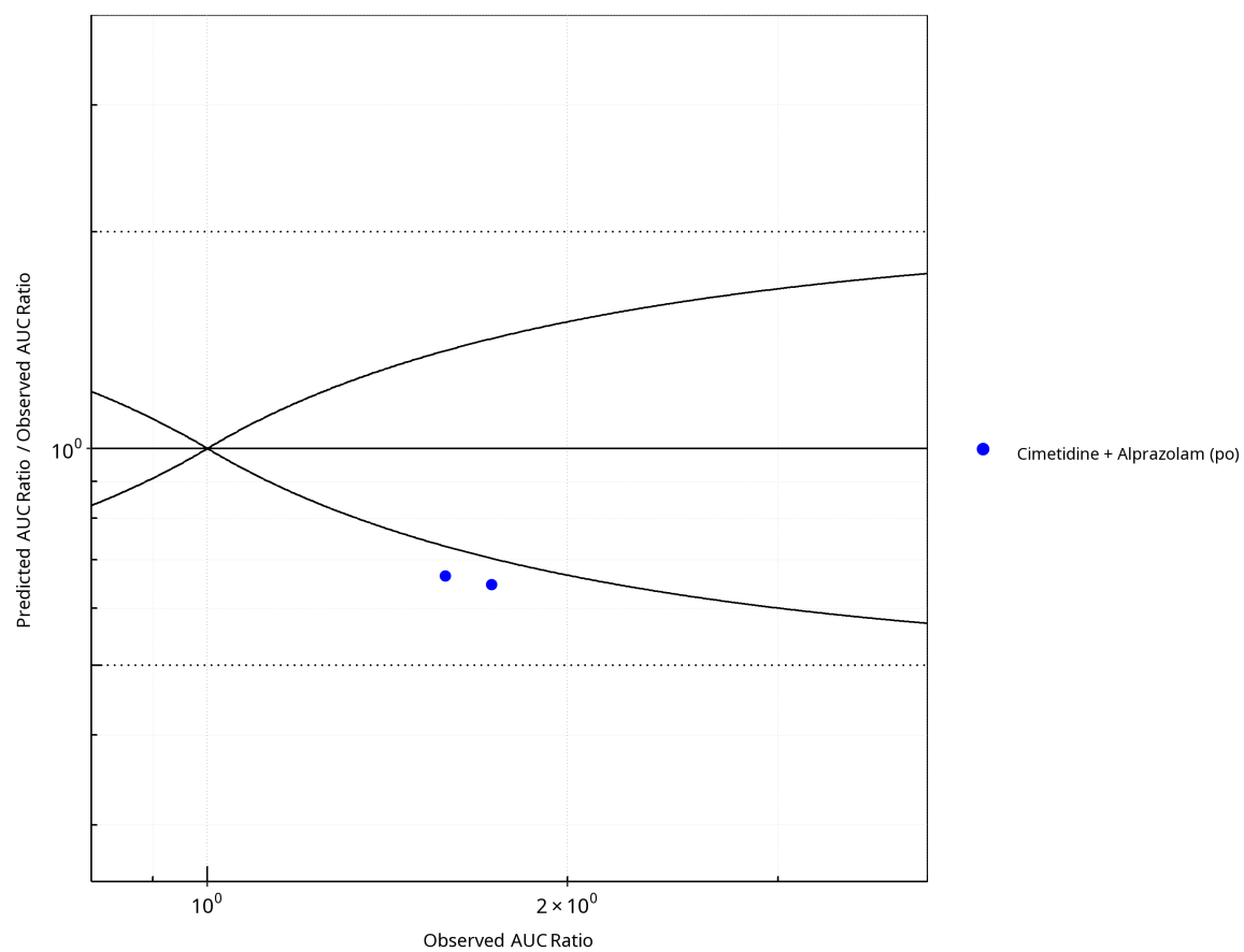
Figure 1-10: Plot. Perpetrator: Cimetidine. Predicted/Observed vs. Observed AUC Ratio. ( \delta = 1 in Guest et al. formula)
