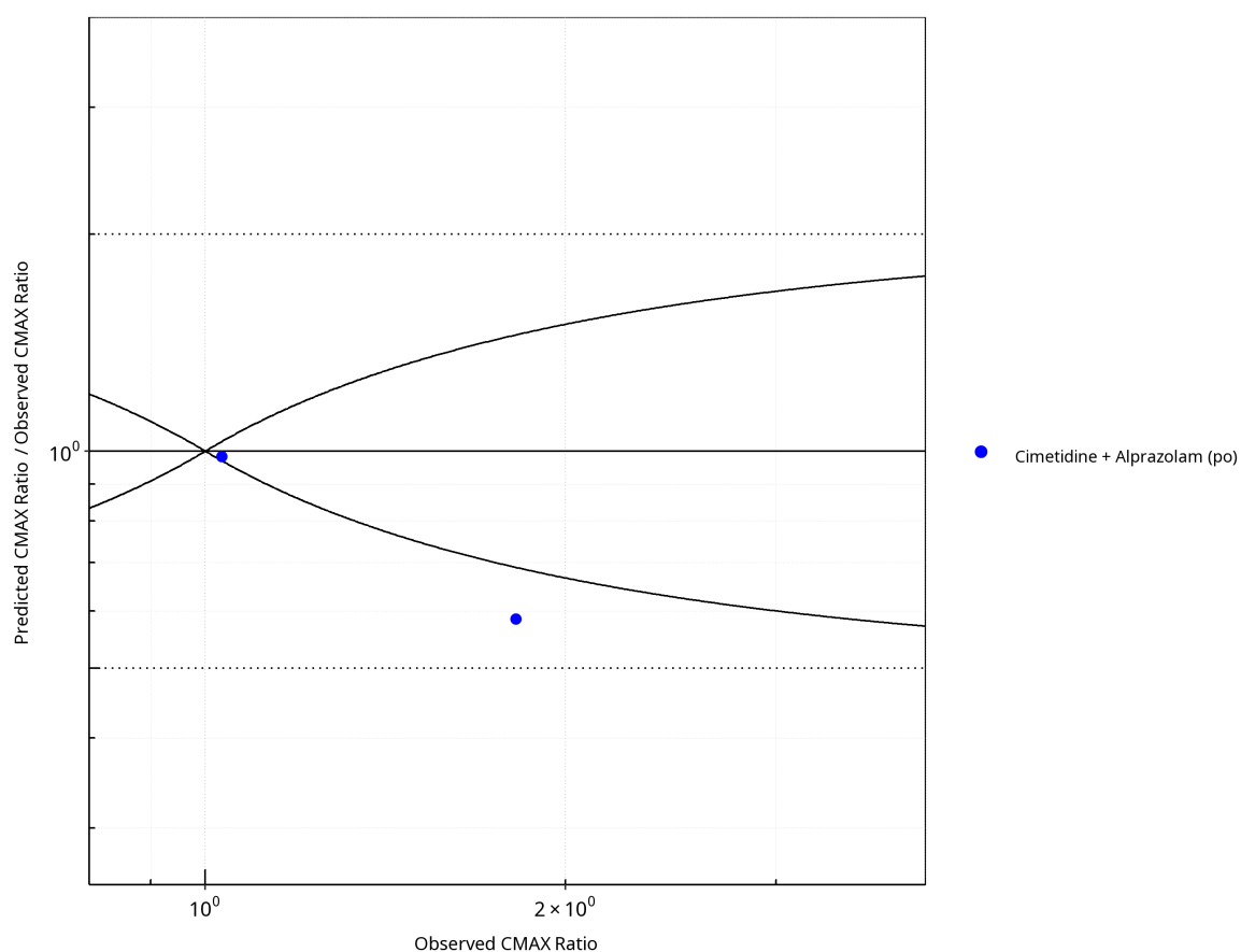
Figure 1-4: Plot. Predicted/Observed vs. Observed CMAX Ratio. ( \delta = 1 in Guest et al. formula)
