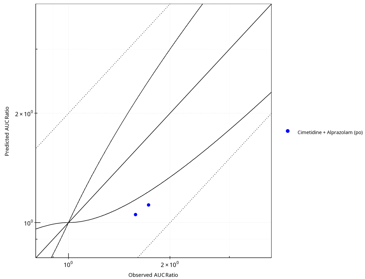
Figure 1-5: Plot. Mechanism: Reversible Inhibition. Predicted vs. Observed AUC Ratio. ( \delta = 1 in Guest et al. formula)
