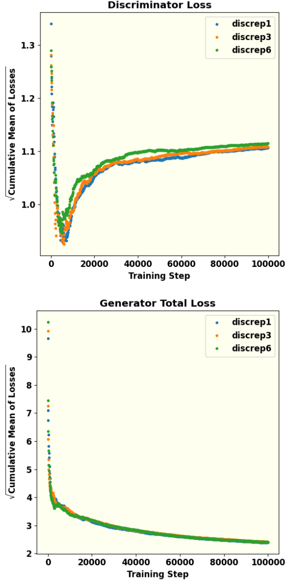
FIG. 7.— These figures show the effect of the ratio of episodes of Discriminator training per every episode of Generator training. This hyperparameter is termed Discriminator repetition or (discrep) in the figures. The square root of the cumulative mean of the losses are plotted against the training steps for 3 values of this ratio. Understandably, this ratio has a higher impact on the Discriminator loss than the Generator loss. Equal number of episodes of training produces minimum cumulative loss of the Discriminator. The dip in the Discriminator loss during the initial phases of its training can be interpreted as its early success in detecting “fake” (or generated) images because of a poorly trained Generator. With gradual training of the Generator, the success rate of the Discriminator decreases and eventually approaches saturation with equal probability of being successful in telling “fake” from real. The continual decrease and eventual saturation of the Generator loss is a result of its training to generate better images with increasing number of steps.
