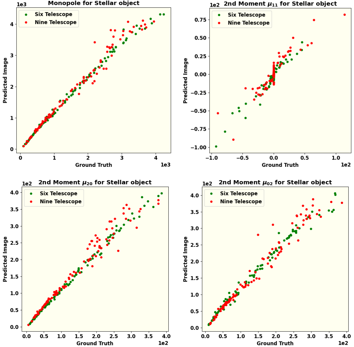
FIG. 10.— Comparison of moments of the predicted images with those of the ground-truth images. Continued on the next page.
