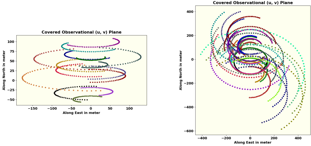
FIG. 2.— The tracks of the baselines of the two hypothetical II observation facilities shown in fig. 1 generated (synthetically) due to Earth's rotation during one night of simulated II observation. The number of baselines scales as square of number of telescopes in the array thus leading to greater coverage of the observational plane and better image reconstruction prospects.
