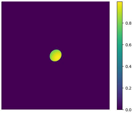
FIG. 3.— This figure shows one of the simulated fast rotating stars (FRS). Brightness is the highest at the poles; gravity darkening is visible along the equator. A total of 31460 such images of FRS with different parameter values have been generated to train the model.
