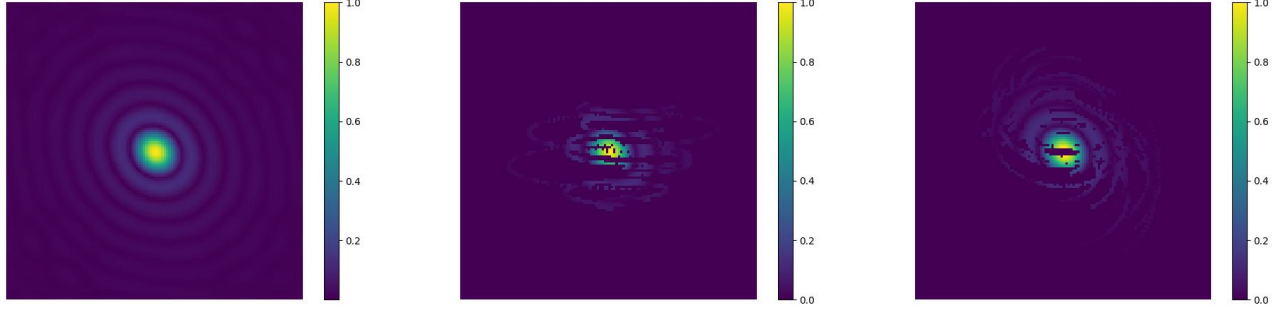
FIG. 4.— The left panel shows the absolute value of the two-dimensional Fast Fourier Transform (FFT) of the source depicted in Fig. 3. It represents the interferometric (u, v) plane intensity distribution that would be generated by an infinite number of baselines (or an infinite number of telescopes) observing the source. The middle and right panels represent the same intensity distribution as sampled along the tracks shown in the left and right panels of Fig. 2 respectively. The middle and right panels reflect the sparse nature of the signal received by a realistic finite number of telescopes and baselines sampled from the full (u, v) plane signal space. All figures are plotted on a linear scale and normalized to the maximum pixel value in each respective figure.
