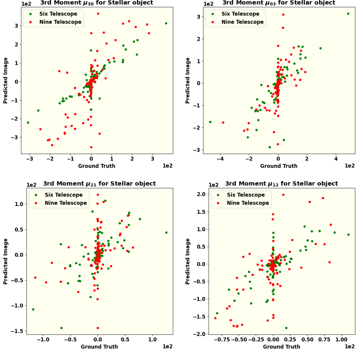
FIG. 10.— Continued. The panels of this figure depict the comparison of moments of predicted images with those of the ground-truth images. The predicted images are generated by our trained cGAN model vis. a vis. the ground-truth images in the two Test Sets. The green and red dots represent the moments of the FRSs generated from II observations with arrays of N_T = 6 and N_T = 9 IACTs, respectively. The small scatter in the moments of the predicted images indicates balanced training of the model. This figure also shows that improvement in (u, v) coverage dominates over the number of baselines.
