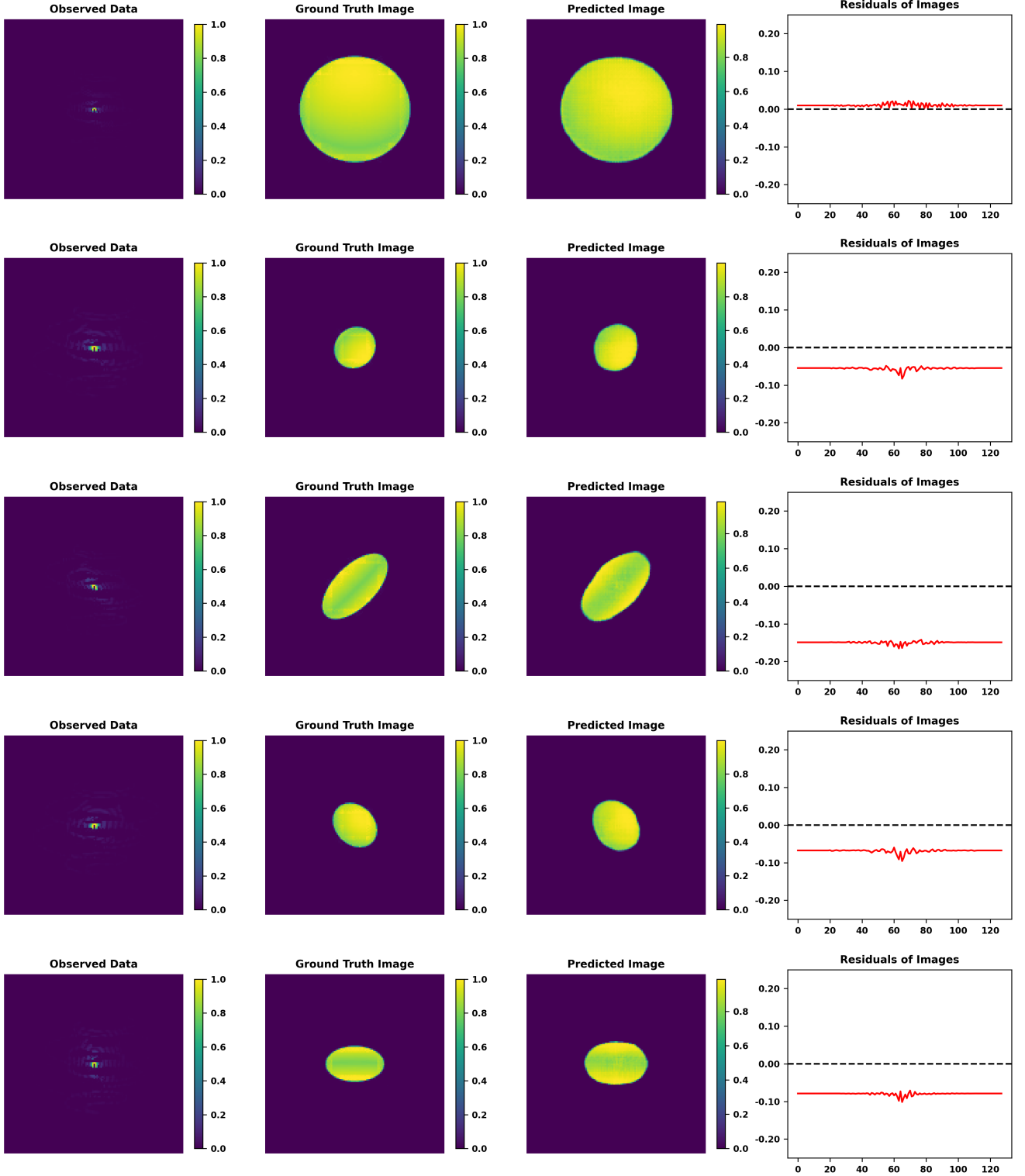
FIG. 8.— Example results of image reconstruction using the cGAN model along with the II observations simulated in this work. Each row in this figure represents the results for a hypothetical fast-rotating star. The left panel represents the sparse II pattern obtained by the simulated observation of the star using the array of N_T = 6 IACTs illustrated in the left panel of Fig. 1. This image acts as the “condition” part of the data input to the cGAN model. The second panel from left displays the real image, or ground truth, which the Discriminator uses to distinguish from the images generated by the Generator. The data generated for training, validation and testing of the cGAN model is a merge of this image and its II pattern presented in the left panel. The third panel is the reconstructed image, or the predicted image, produced by the trained GAN model. The fourth and the last panel shows the 1D-residuals between the ground truth and the predicted image in the (u, v) plane. The x-axis of this panel represents the horizontal pixel coordinate and the y-axis shows the residual intensity value at the respective pixel.
