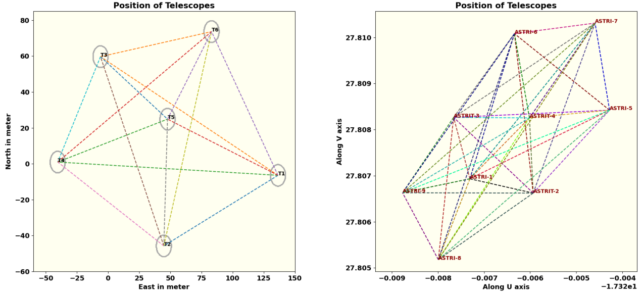
FIG. 1.— A schematic representation of a hypothetical observation facility with an array of N_T = 6 Imaging Atmospheric Cherenkov Telescopes (IACs) (left panel) and N_T = 9 IACs that mimic the telescope configuration of ASTRI Scuderi et al. (2022) (right panel). In the work presented here, these two sets of arrays are used in simulating the II observation of the fast rotators.
