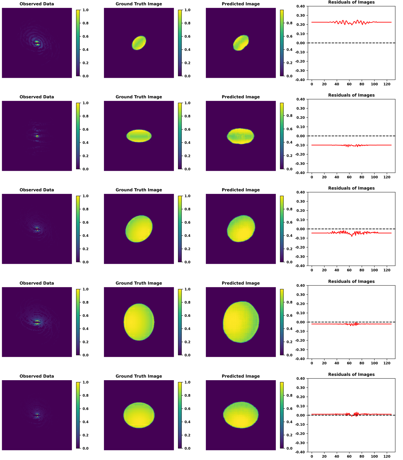
FIG. 9.— Example results of image reconstruction using the cGAN model (as presented in Fig. 8), but with the II simulations carried out with the array of N_T = 9 as shown in the right panel of Fig. 1. Panel labels are as described in the caption of Fig. 8.
