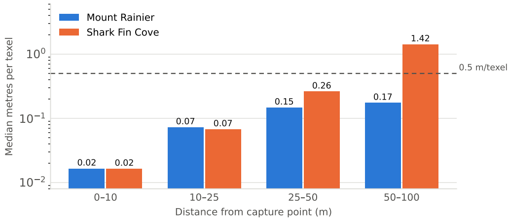
Figure 15: Texture resolution against distance, log scale. The two captures are indistinguishable within 25 m; beyond it Shark Fin degrades far faster, because a clifftop camera places most of its surface near the horizon where equirectangular compression is worst. Above roughly 0.5 m per texel we take the ground to read as smeared.
