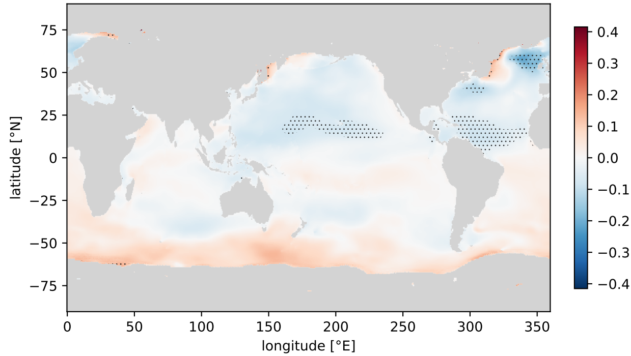
SSP5-8.5 – historical: \Delta mean
