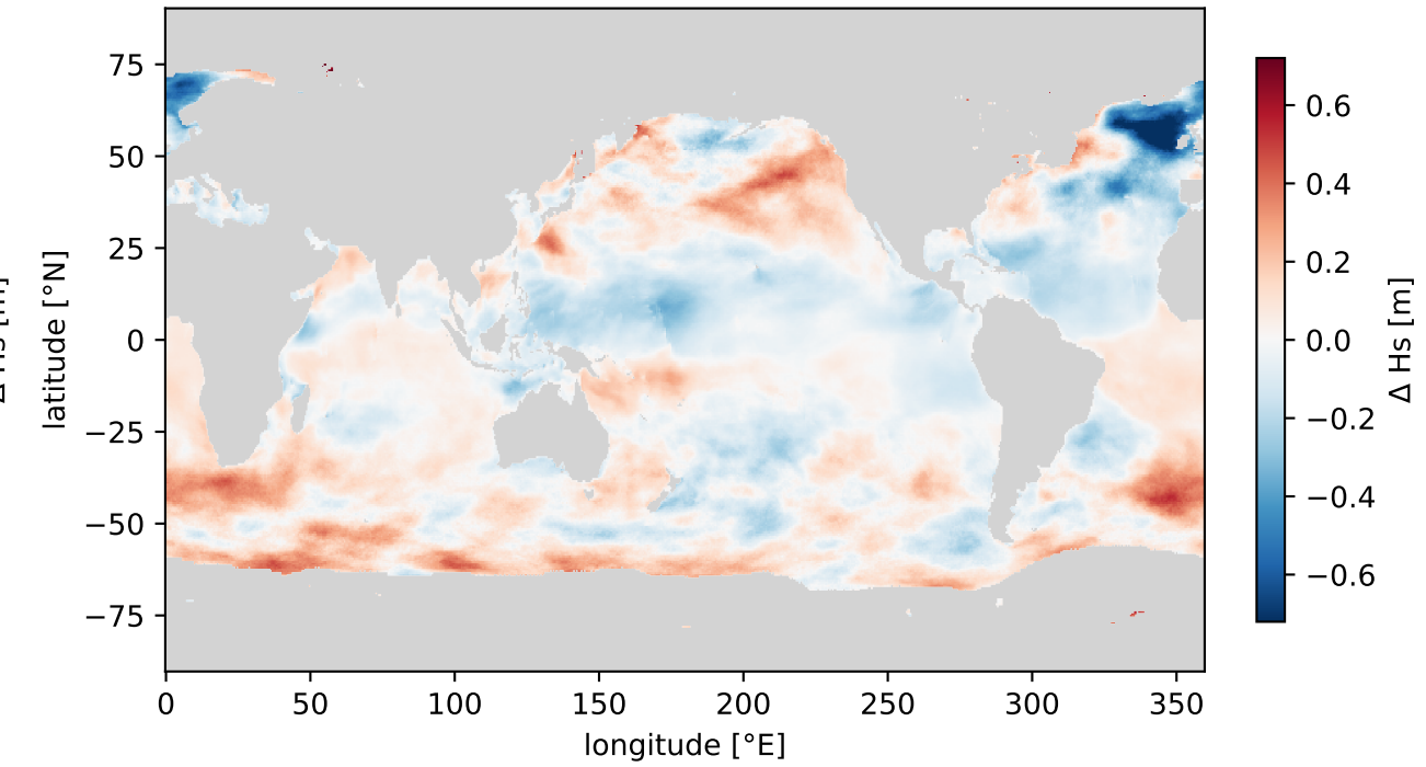
SSP5-8.5 – historical: \Delta 99th percentile
