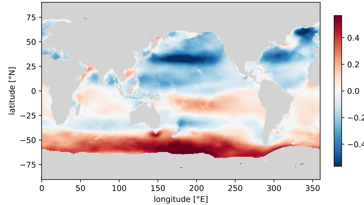
SSP5-8.5 – historical: \Delta 90th percentile
