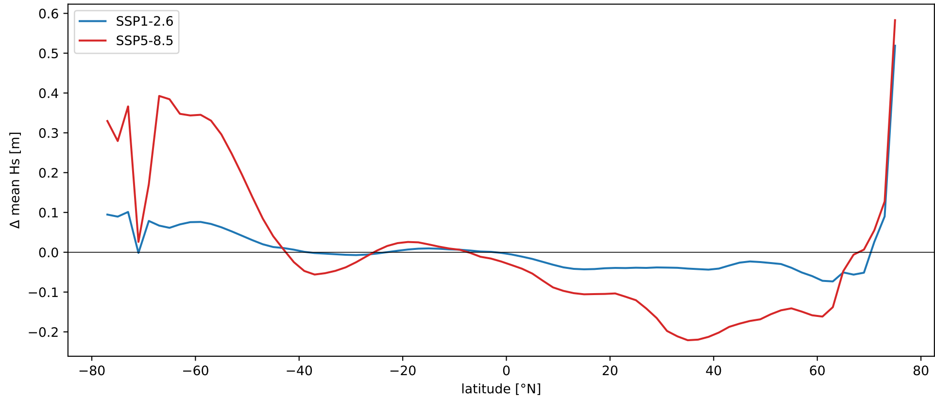
Zonal-mean change in mean Hs (masked points excluded)
