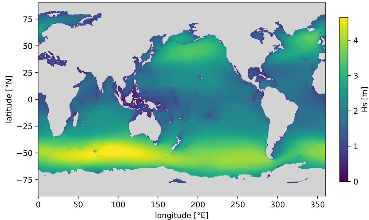
historical 1985-2014: mean Hs
