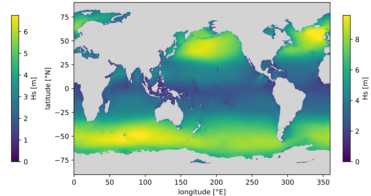
historical 1985-2014: 99th percentile Hs
