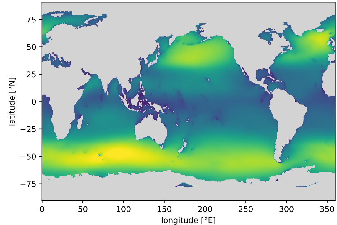
historical 1985-2014: 90th percentile Hs
