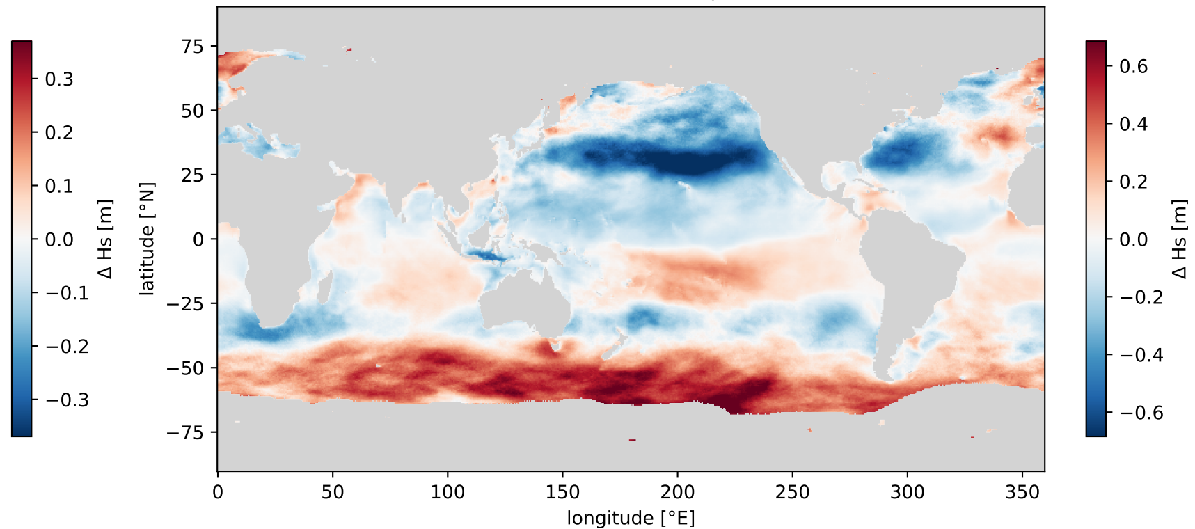
SSP5-8.5 – SSP1-2.6: 99th percentile Hs
