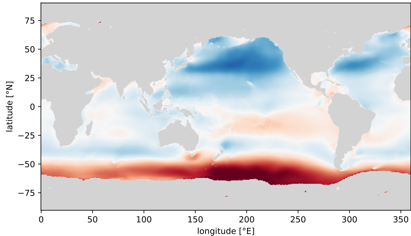
SSP5-8.5 – SSP1-2.6: mean Hs
