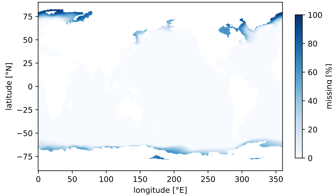
historical (1985-2014): time missing
