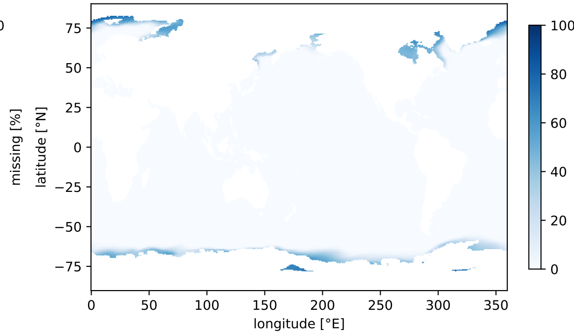
ssp126 (2071-2098): time missing
