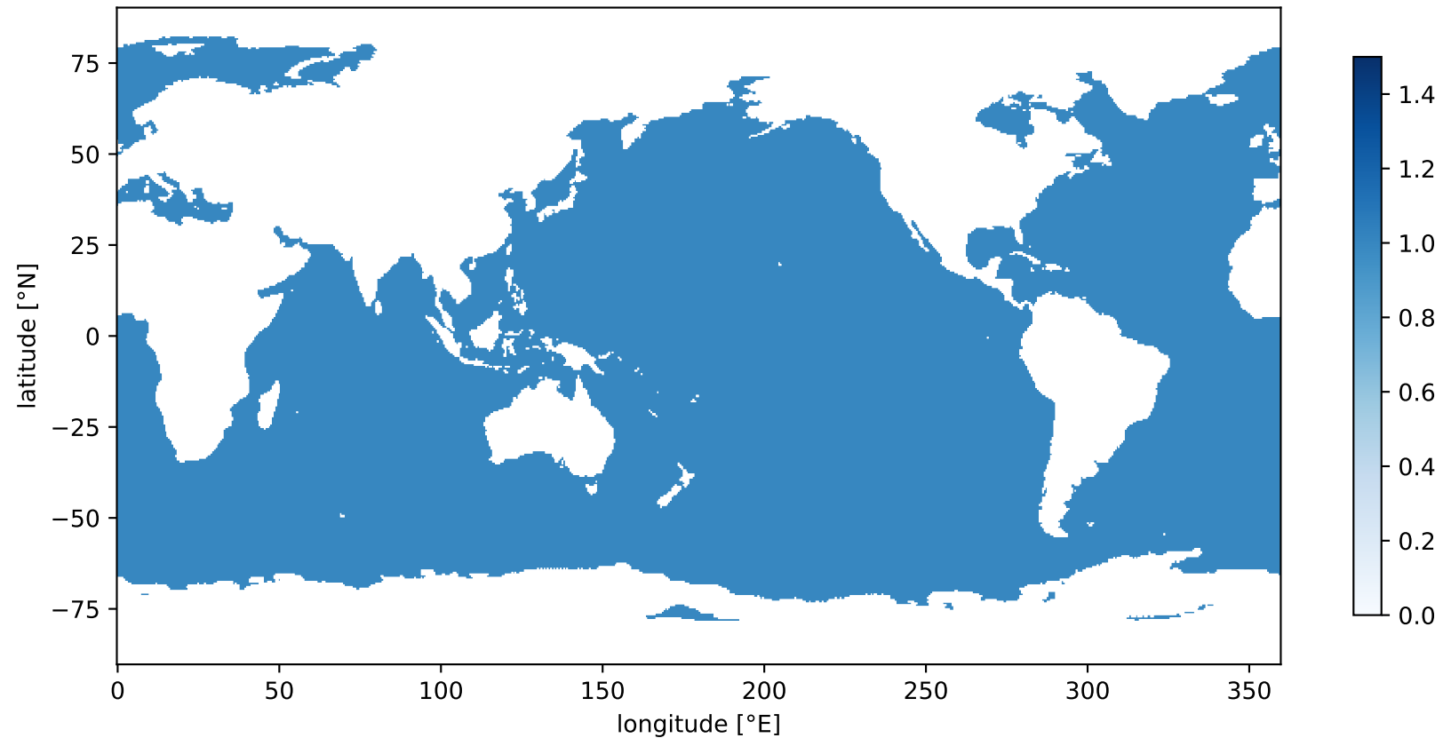
The 142,868 sea points of the 0.5° grid
