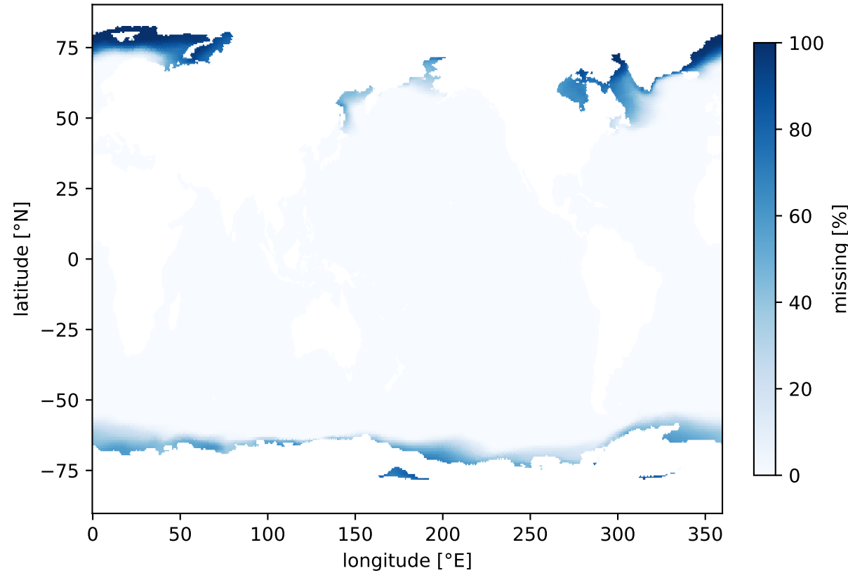
historical: share of time steps missing
