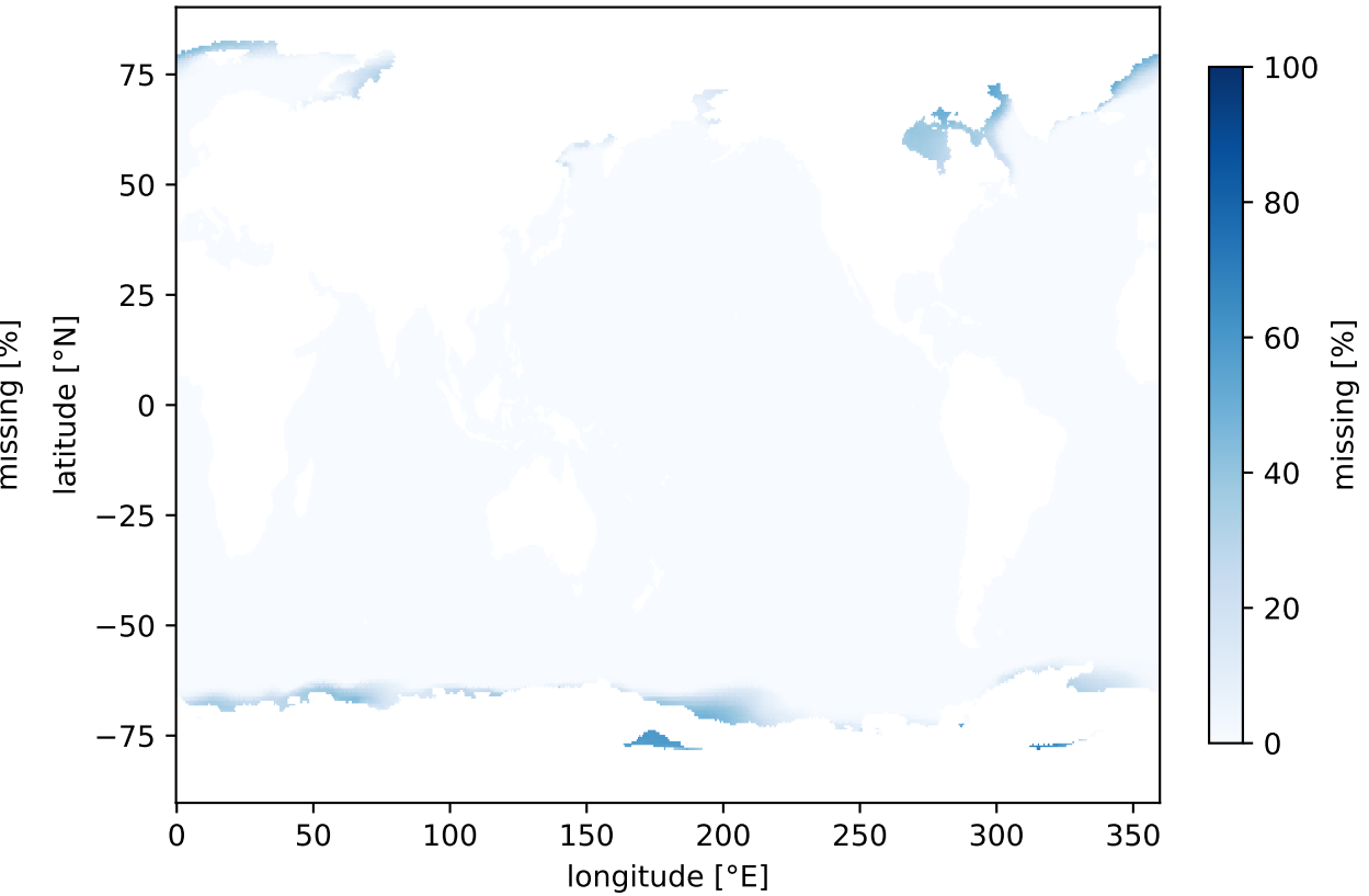
ssp585: share of time steps missing
