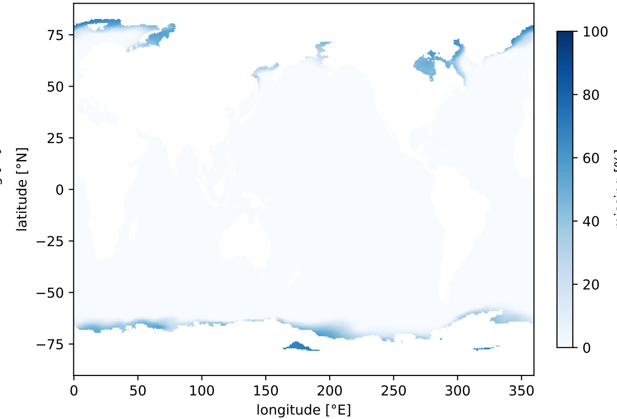
ssp126: share of time steps missing
