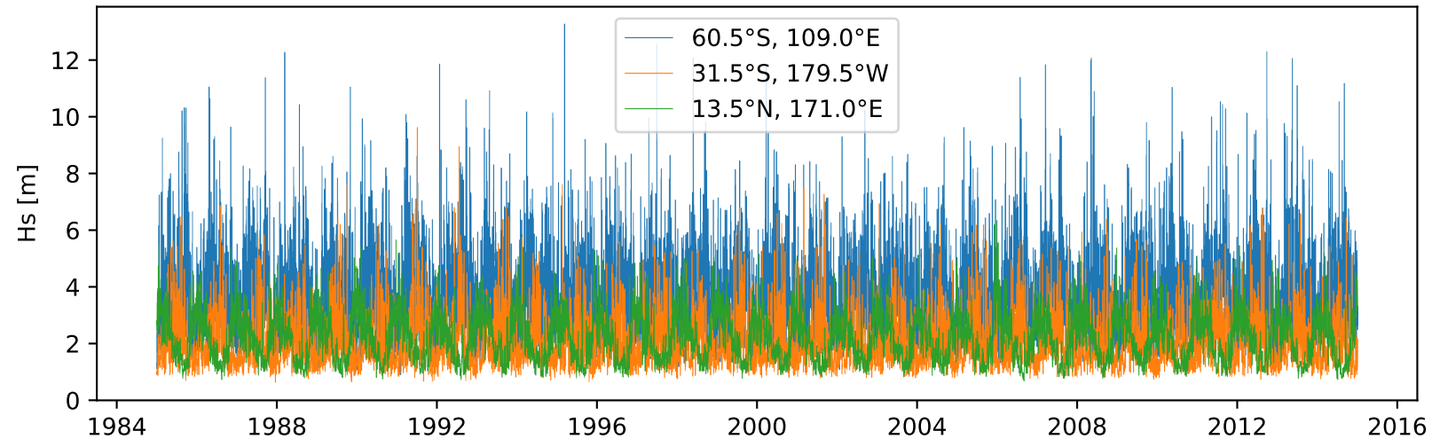
Significant wave height, 3-hourly (time axis assumed to start 1 Jan 1985)
