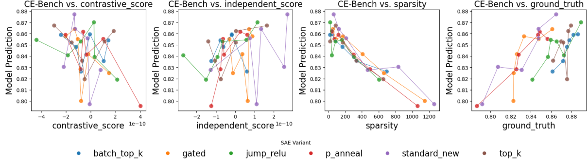
Figure 7: Ablation — Mean Pooling Strategy. Using mean pooling results in highly inconsistent and noisy predictions, with no clear correlation between CE-Bench scores and the contrastive or independent metrics. This indicates that averaging across all neurons fails to highlight the most semantically informative features.
