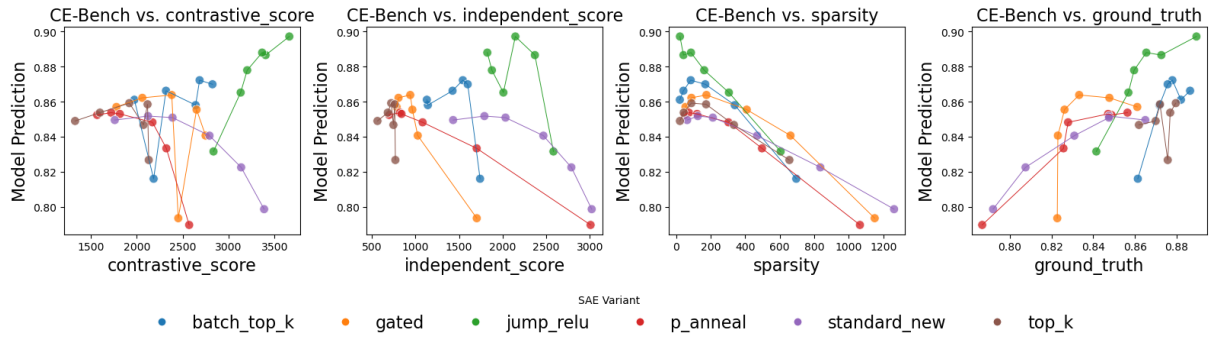
Figure 8: Ablation — Outlier Count Pooling Strategy. This strategy yields a misleading negative correlation between predicted interpretability and independent scores, contradicting CE-Bench's core assumption that high subject-specific activation deviation implies stronger interpretability. Thus, outlier count proves suboptimal.
