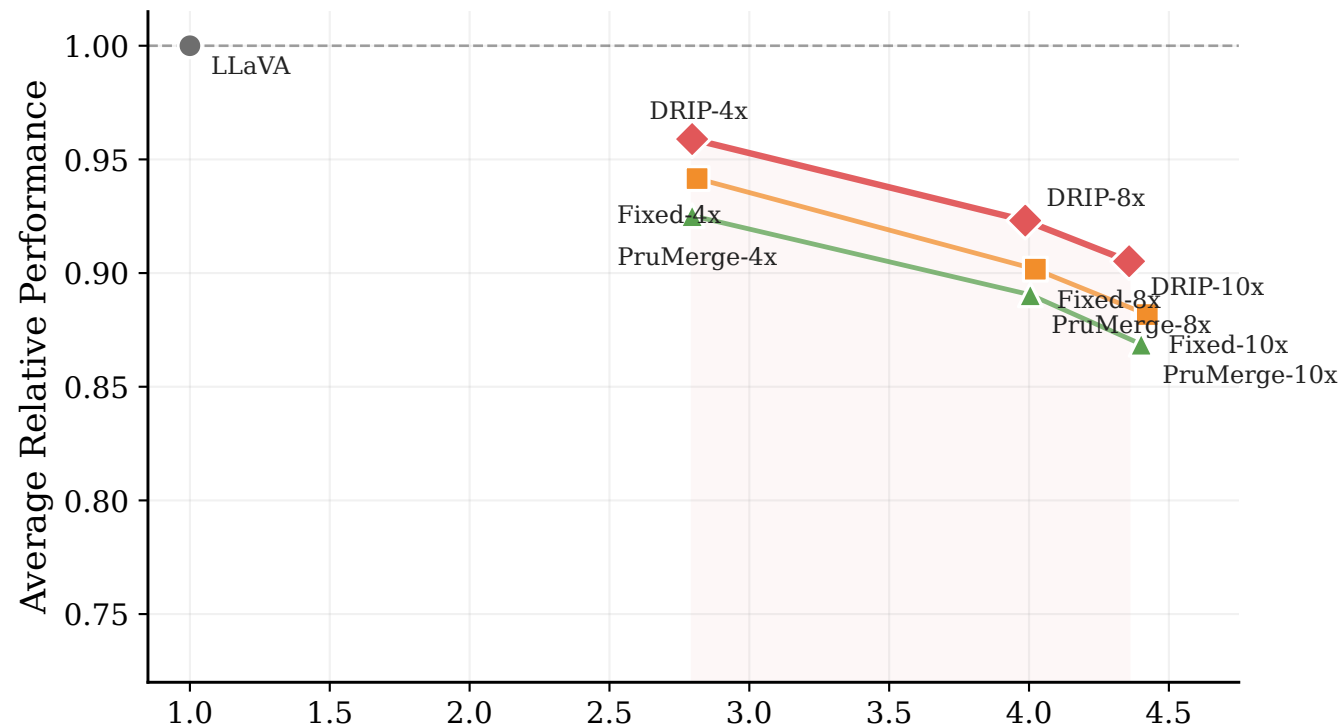
Overall Performance
