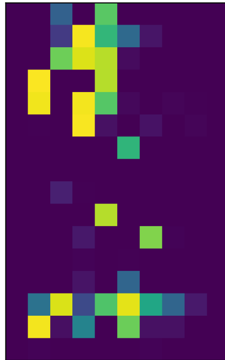
text_dreams: 16×10
