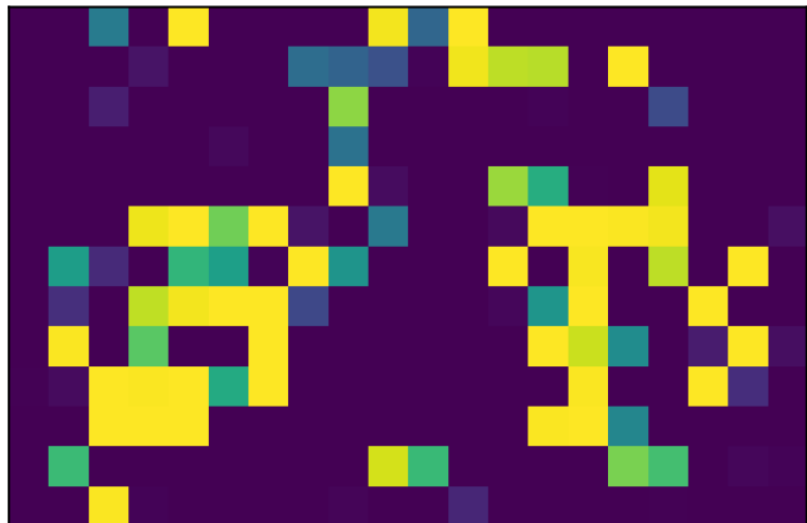
skiing: 13×20
