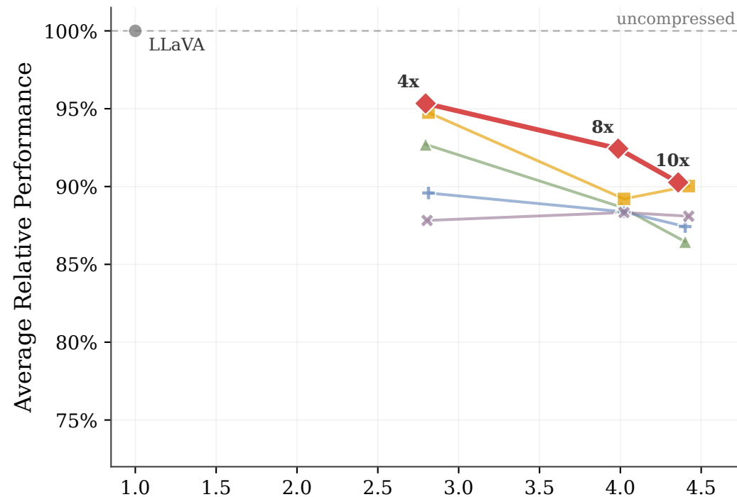
Overall Performance
