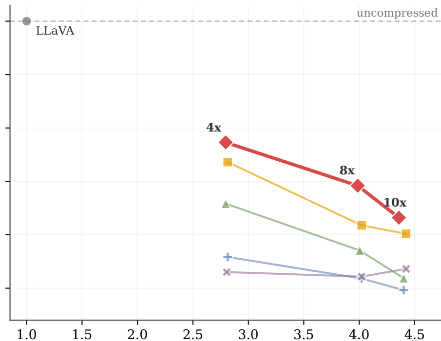
OCR Performance
