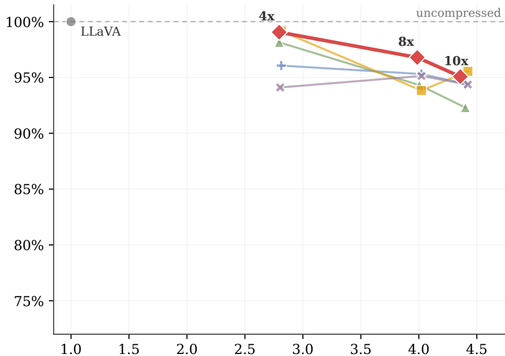
Coarse-grained QA Performance
