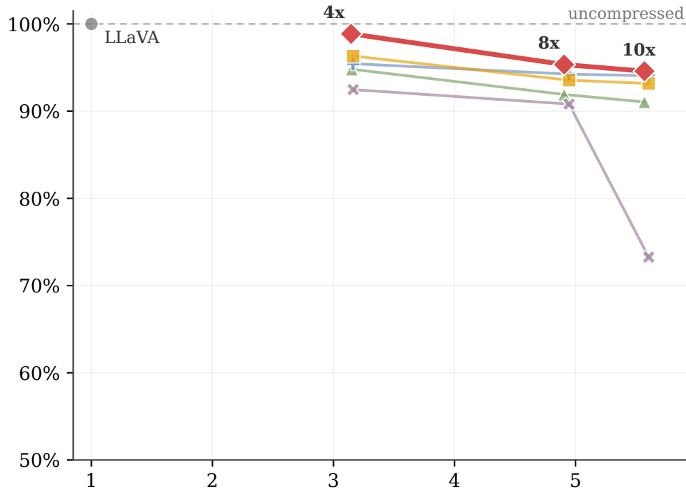
Coarse-grained QA Performance
